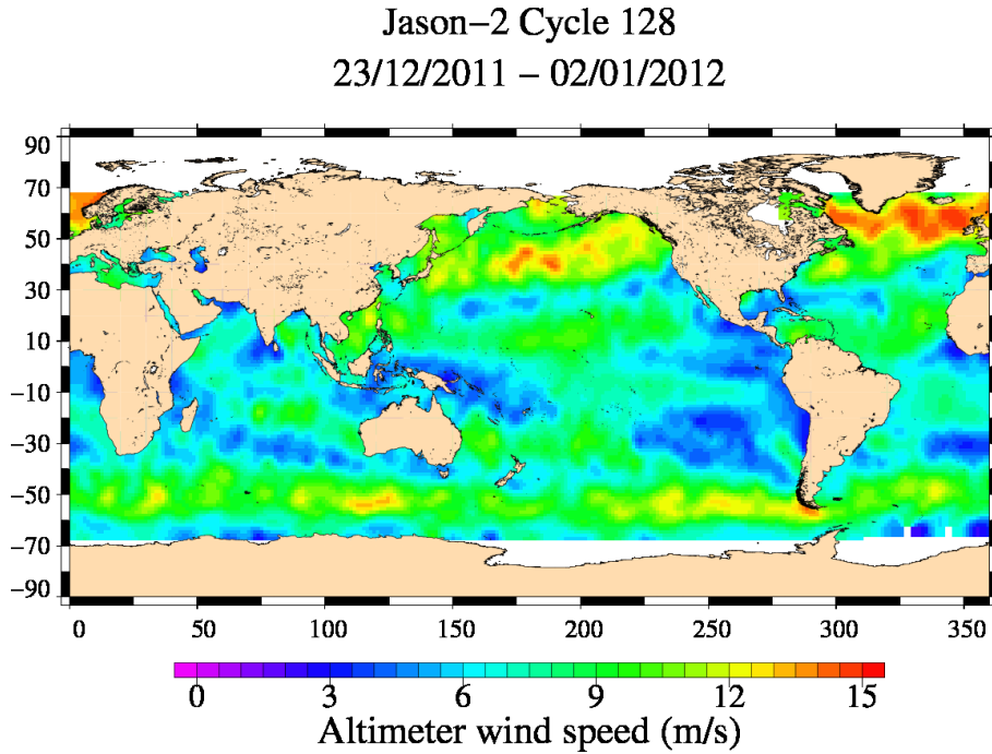
FIG. 9 – Altimeter wind speed for cycle 128.
