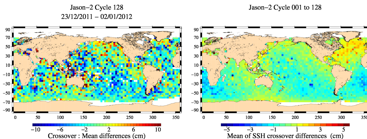
FIG. 13 – Mean SSH at crossovers for cycle 128 (left) and over the whole Jason-2 period (right).
