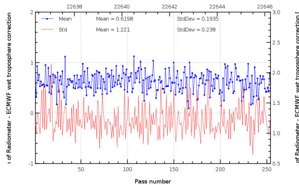
FIG. 11 – Pass monitoring of wet troposphere differences between radiometer and ECMWF model for Jason-2 cycle 128.
