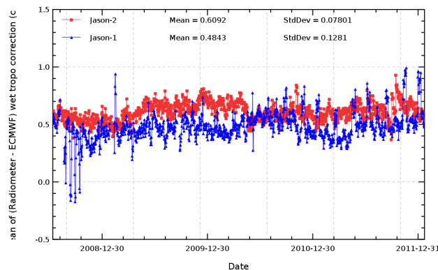
FIG. 12 – Daily monitoring of wet troposphere differences between radiometer and ECMWF model
