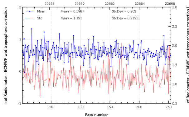
FIG. 11 – Pass monitoring of wet troposphere differences between radiometer and ECMWF model for Jason-2 cycle 130.
