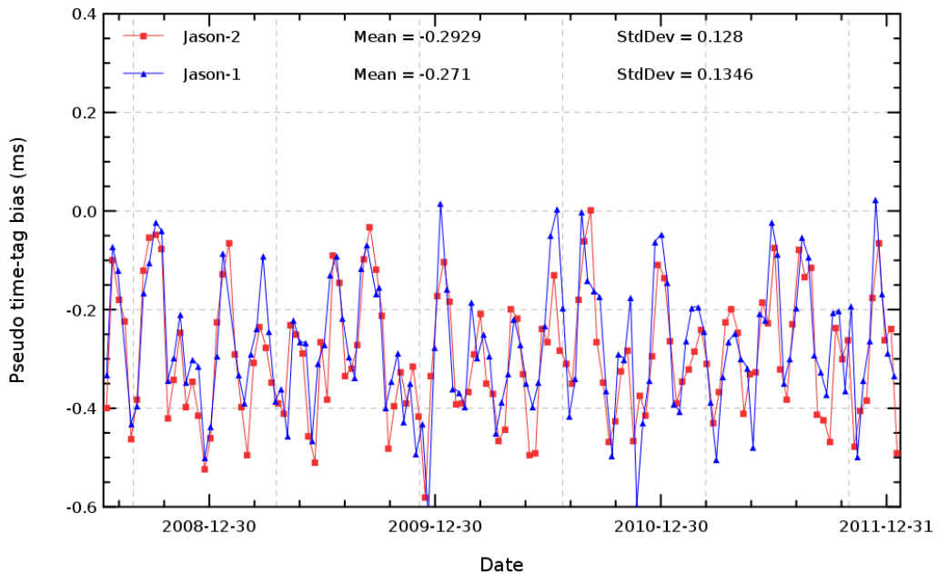
FIG. 16 – Cyclic monitoring of pseudo time tag bias for Jason-1 and Jason-2.
