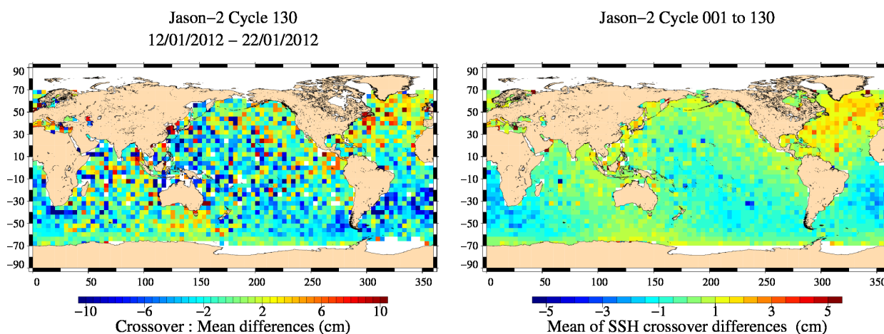
FIG. 13 – Mean SSH at crossovers for cycle 130 (left) and over the whole Jason-2 period (right).
