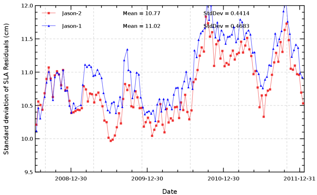
FIG. 21 – Cyclic monitoring standard deviation of along track SLA for Jason-1 and Jason-2.
