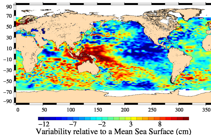
FIG. 18 – Sea level anomaly relative to MSS for cycle 130.
