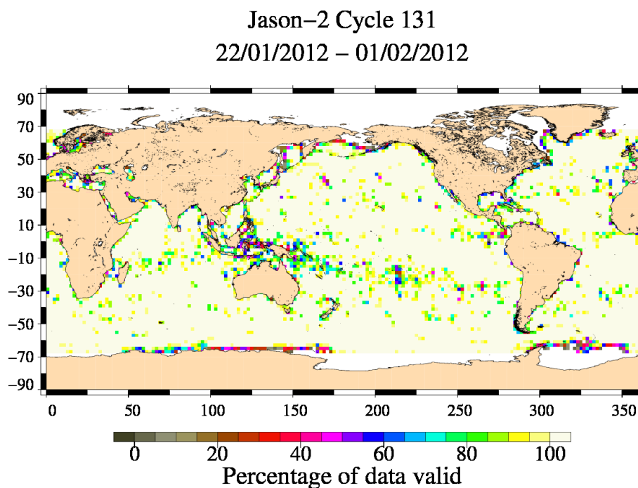
FIG. 3 – Percentage of valid measurements for cycle 131.
