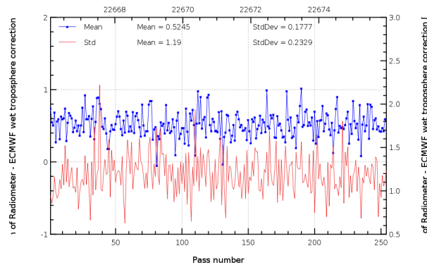
FIG. 11 – Pass monitoring of wet troposphere differences between radiometer and ECMWF model for Jason-2 cycle 131.
