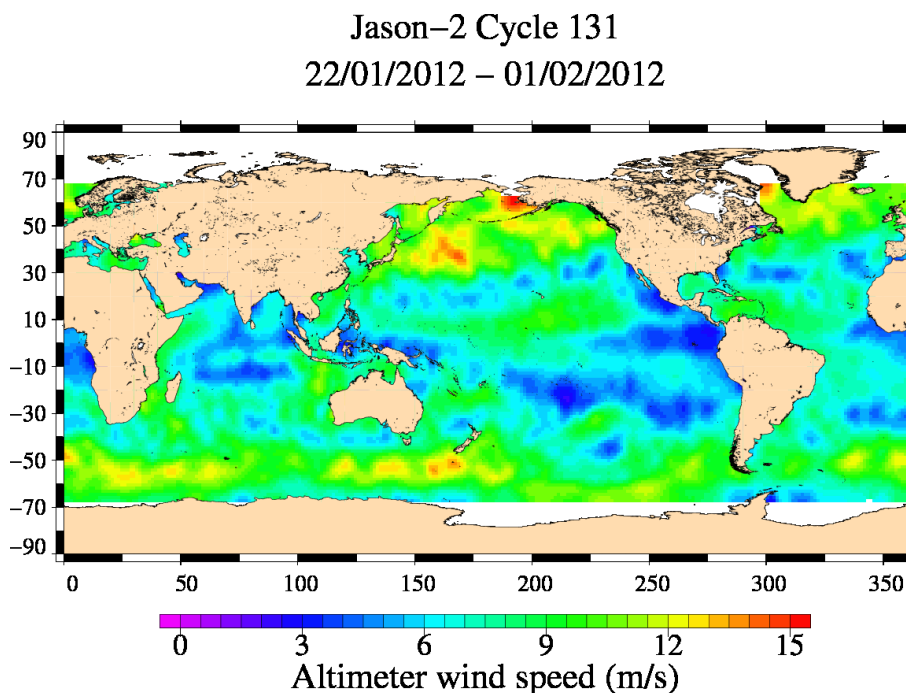
FIG. 9 – Altimeter wind speed for cycle 131.
