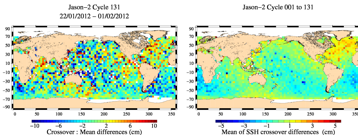
FIG. 13 – Mean SSH at crossovers for cycle 131 (left) and over the whole Jason-2 period (right).
