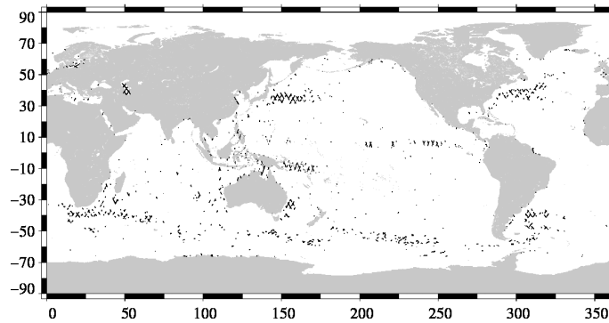
FIG. 19 – Differences higher than a 30 cm threshold for cycle 133.
