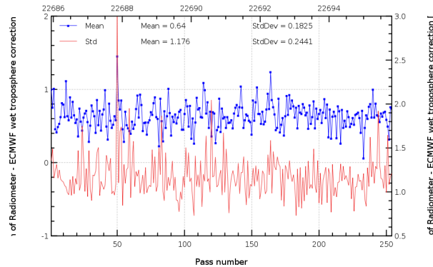
FIG. 11 – Pass monitoring of wet troposphere differences between radiometer and ECMWF model for Jason-2 cycle 133.
