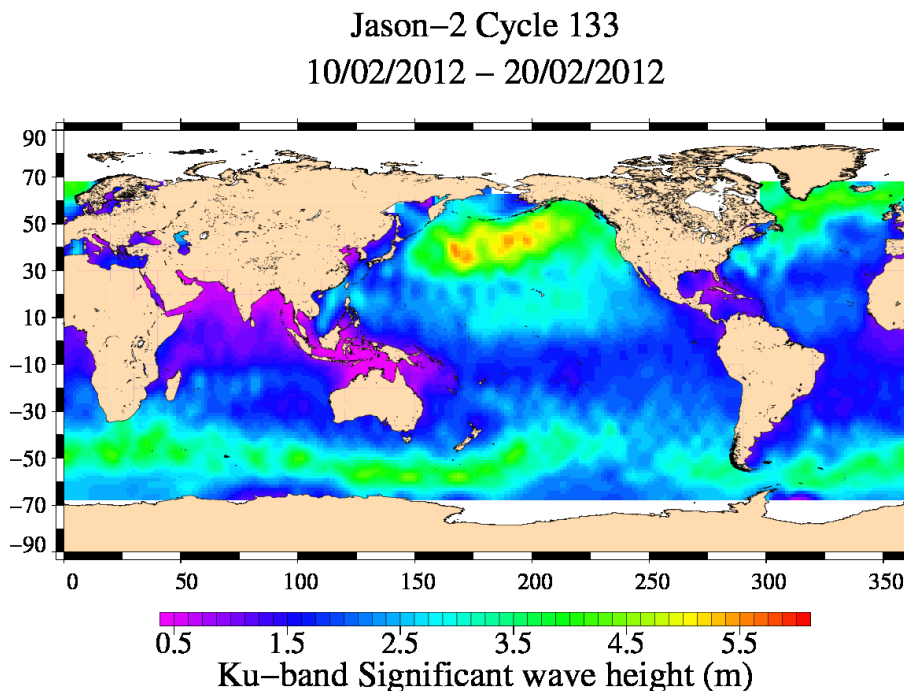
FIG. 5 – Significant wave height for cycle 133.
