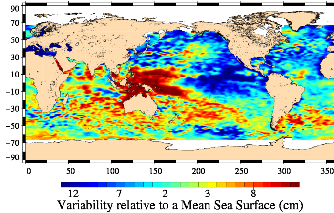
FIG. 18 – Sea level anomaly relative to MSS for cycle 133.
