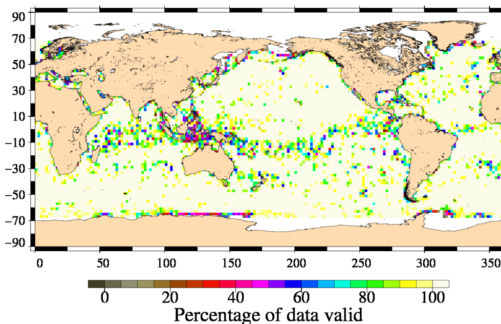
FIG. 3 – Percentage of valid measurements for cycle 133.
