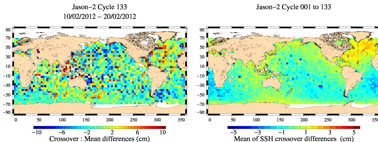
FIG. 13 – Mean SSH at crossovers for cycle 133 (left) and over the whole Jason-2 period (right).
