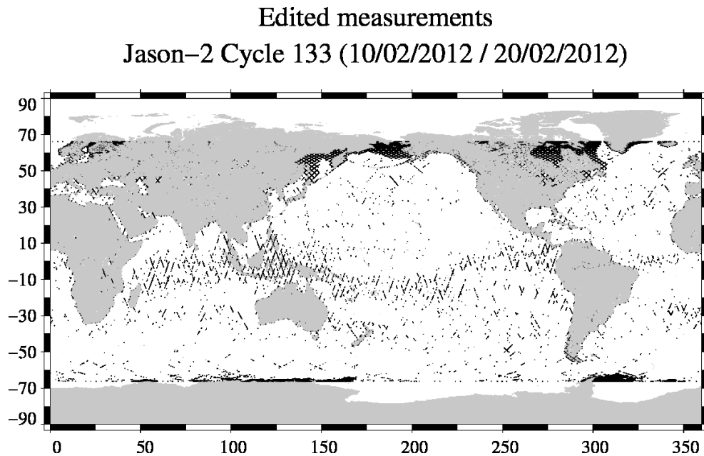
FIG. 2 – Edited measurements for cycle 133.
