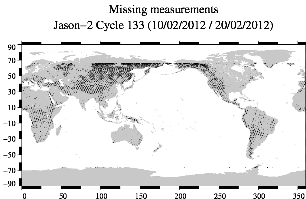
FIG. 1 – Missing measurements for cycle 133.
