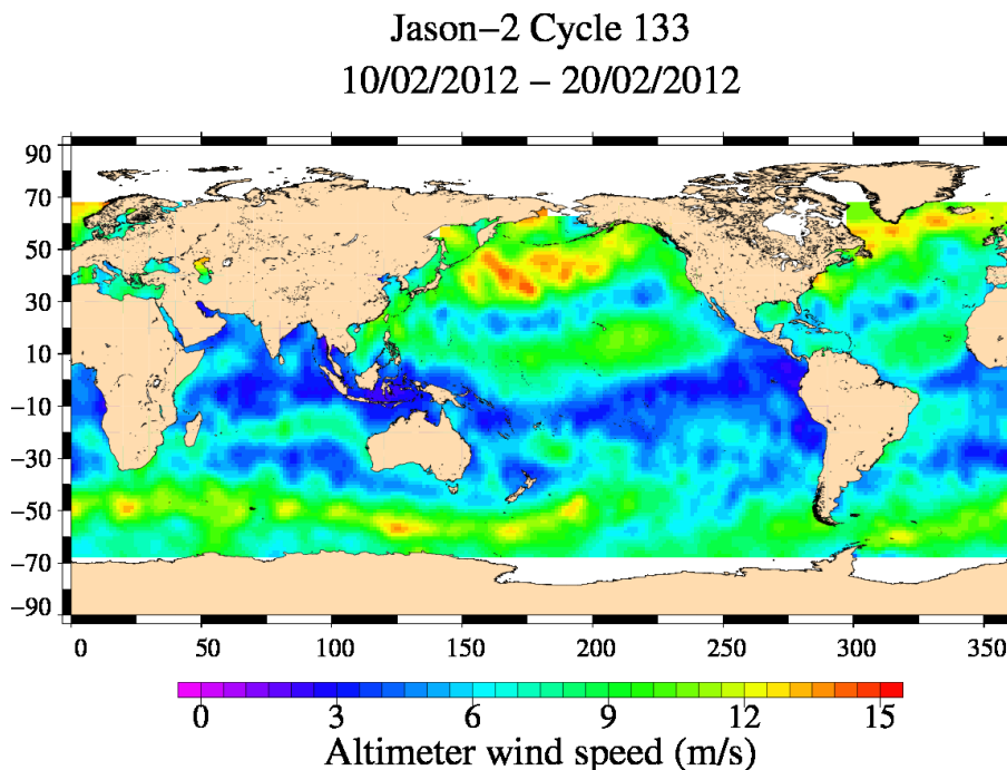
FIG. 9 – Altimeter wind speed for cycle 133.
