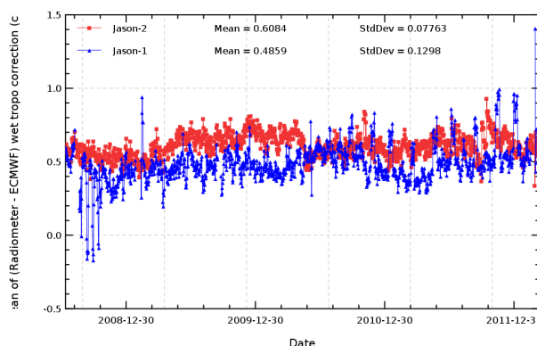
FIG. 13 – Daily monitoring of wet troposphere differences between radiometer and ECMWF model
