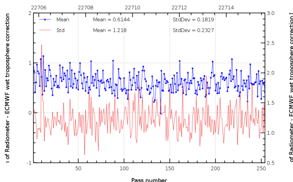
FIG. 12 – Pass monitoring of wet troposphere differences between radiometer and ECMWF model for Jason-2 cycle 135.
