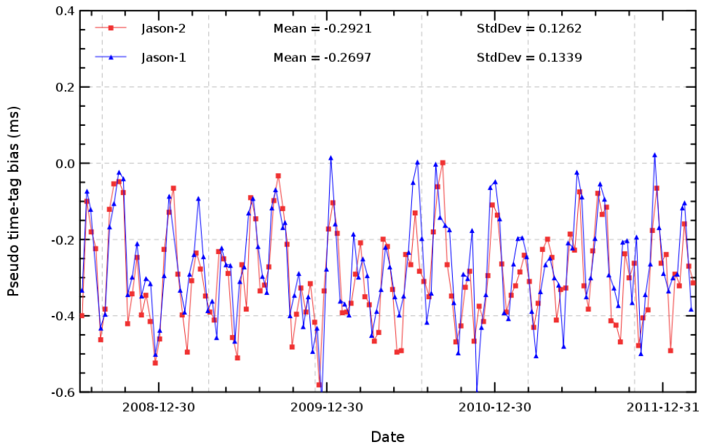
FIG. 17 – Cyclic monitoring of pseudo time tag bias for Jason-1 and Jason-2.
