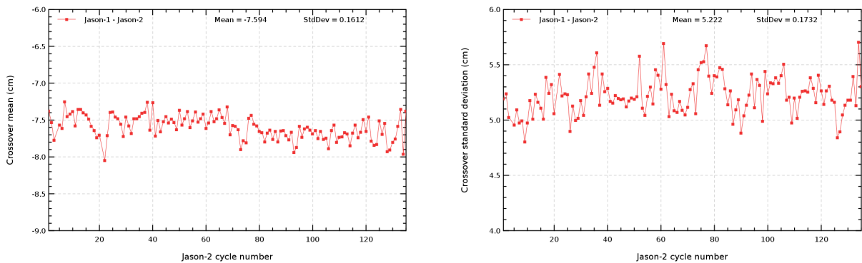
FIG. 16 – Cyclic monitoring of mean (left) and standard deviation (right) of (Jason-1 – Jason-2) SSH differences at crossovers.
