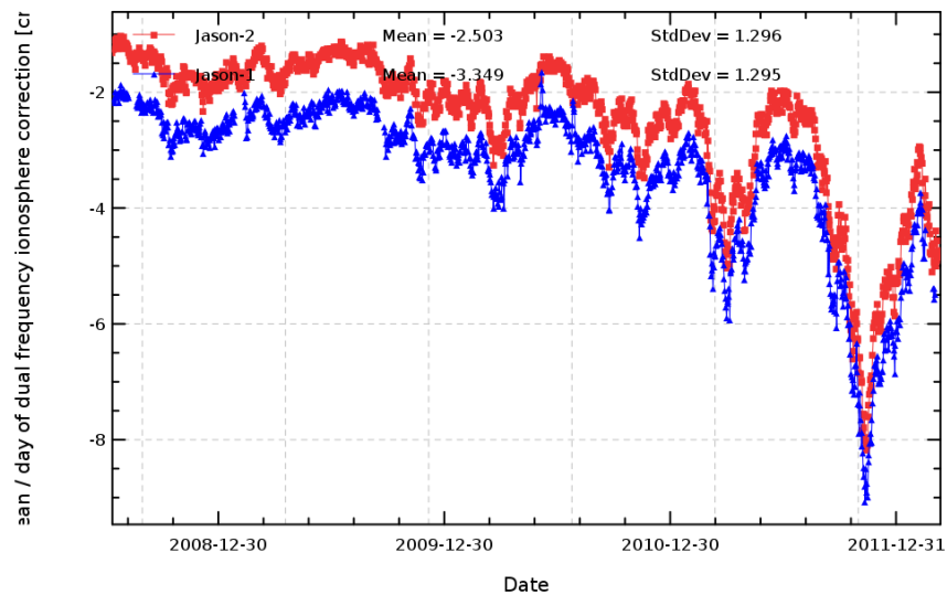
FIG. 9 – Daily monitoring of dual-frequency ionosphere correction for Jason-2 and Jason-1.
