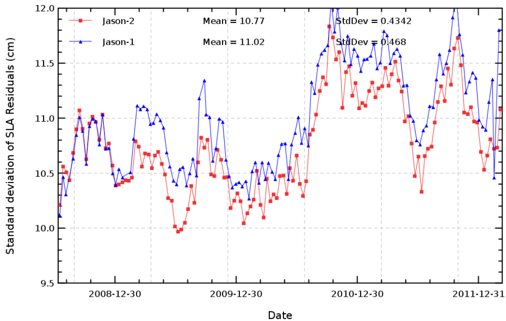
FIG. 22 – Cyclic monitoring standard deviation of along track SLA for Jason-1 and Jason-2.
