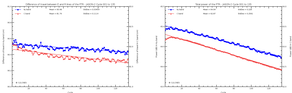
FIG. 5 – Internal path delay (left) and total power of the PTR (right) for Ku- and C-band.
