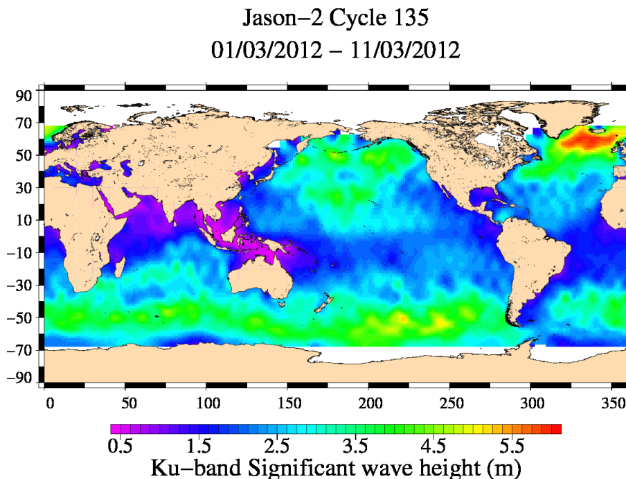
FIG. 6 – Significant wave height for cycle 135.
