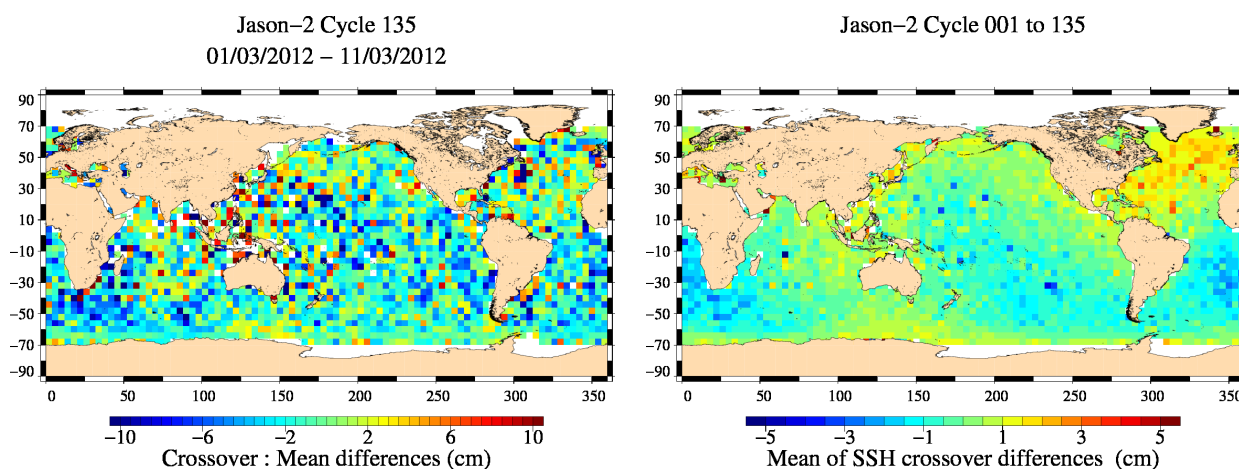
FIG. 14 – Mean SSH at crossovers for cycle 135 (left) and over the whole Jason-2 period (right).
