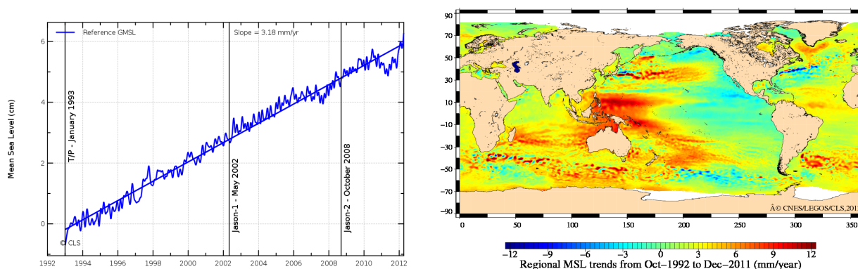
FIG. 23 – Global (left) and regional (right) MSL trends from 1993 onwards.
