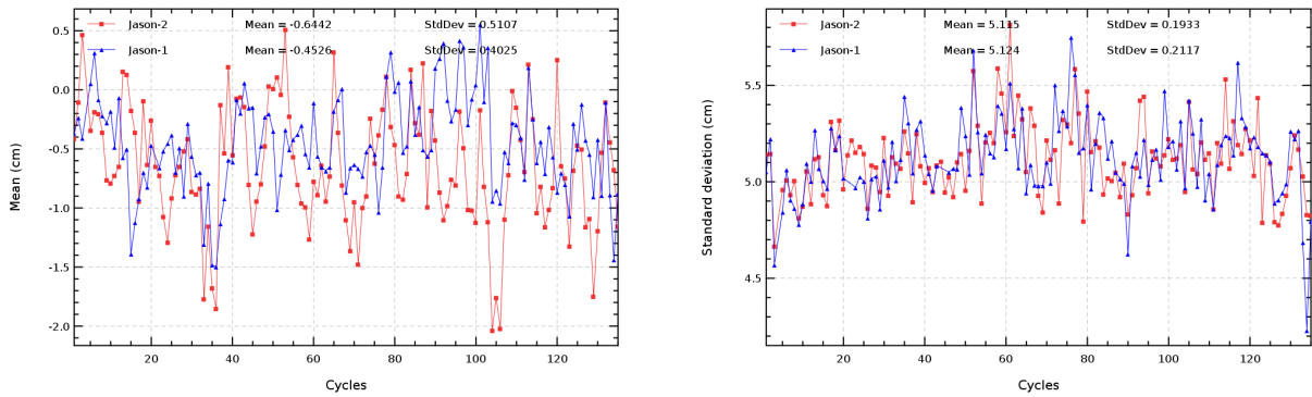
FIG. 15 – Cyclic monitoring of mean (left) and standard deviation (right) of SSH differences at crossovers for Jason-1 and Jason-2.
