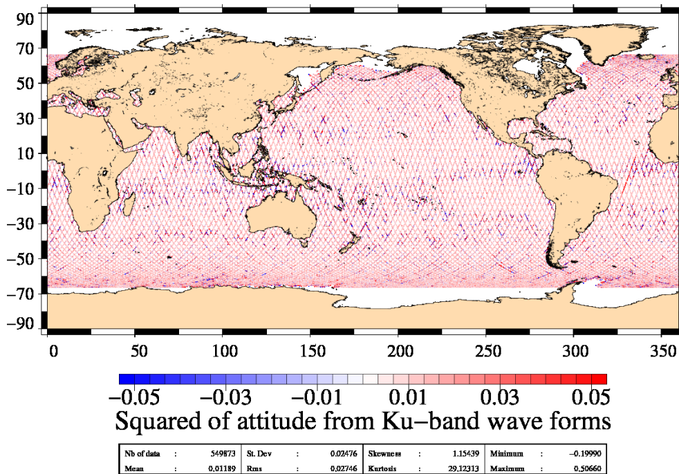
FIG. 4 – Apparent squared mispointing from waveforms for cycle 135.
