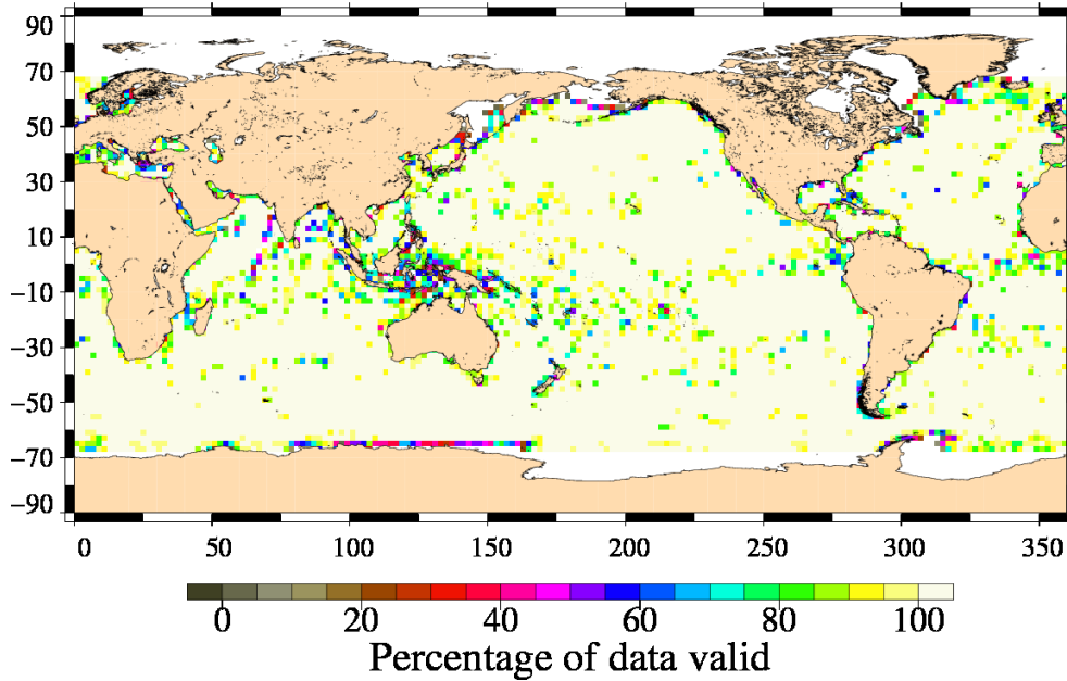
FIG. 3 – Percentage of valid measurements for cycle 135.
