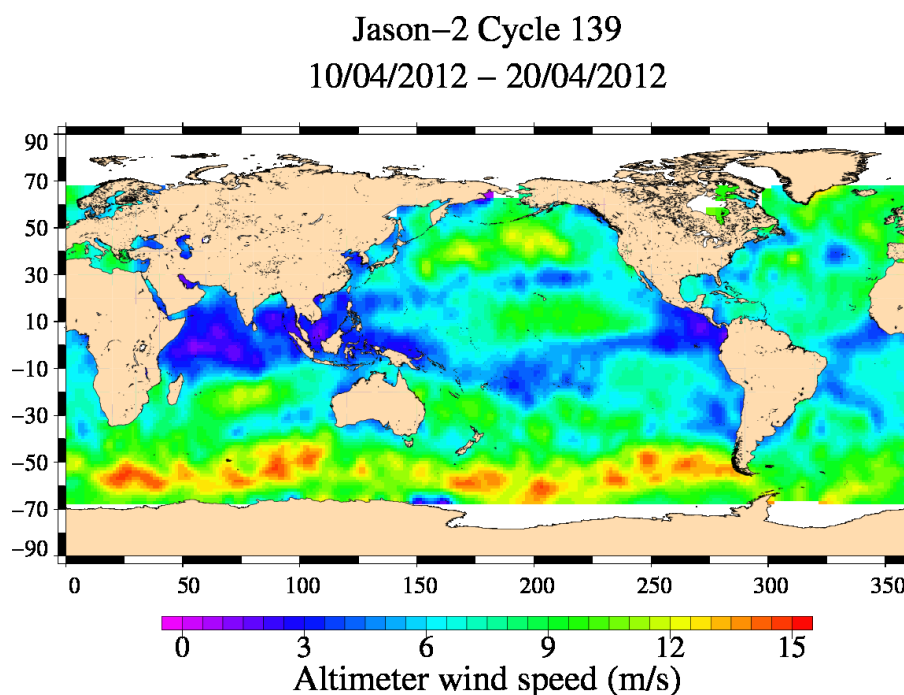
FIG. 9 – Altimeter wind speed for cycle 139.
