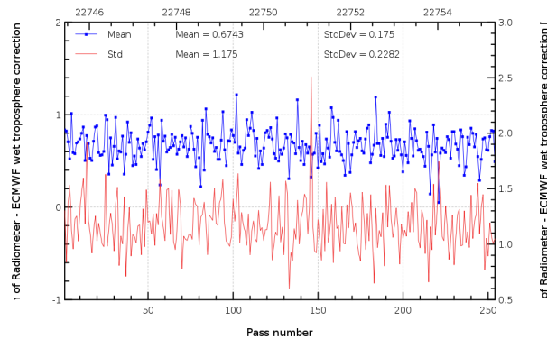
FIG. 11 – Pass monitoring of wet troposphere differences between radiometer and ECMWF model for Jason-2 cycle 139.
