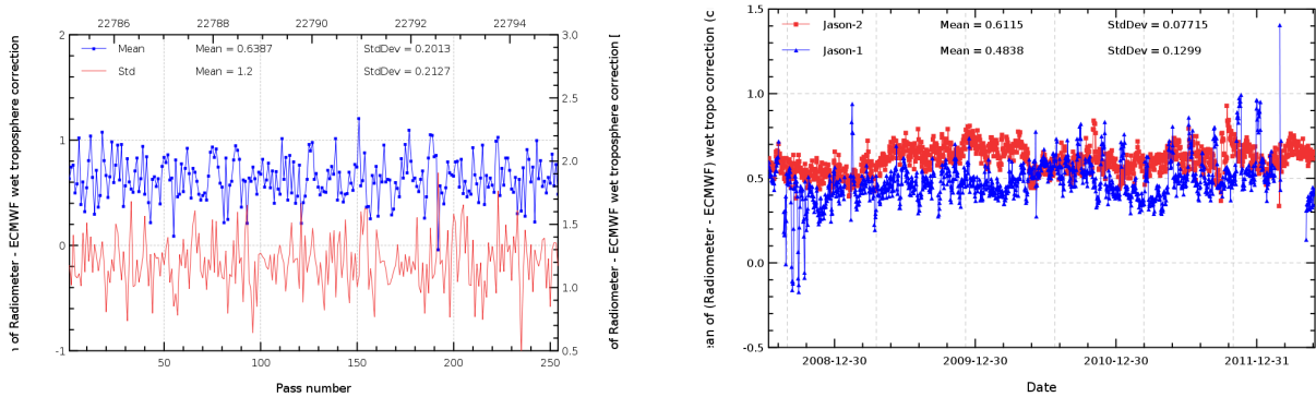
FIG. 11 – Pass monitoring of wet troposphere differences between radiometer and ECMWF model for Jason-2 cycle 143. (left) and Daily monitoring of wet troposphere differences between radiometer and ECMWF model (right).
