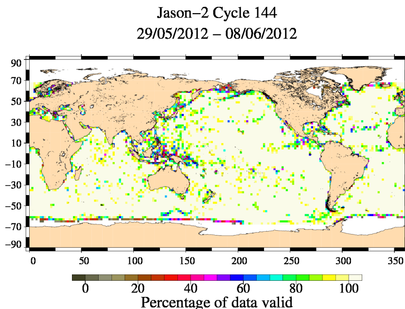
FIG. 3 – Percentage of valid measurements for cycle 144.
