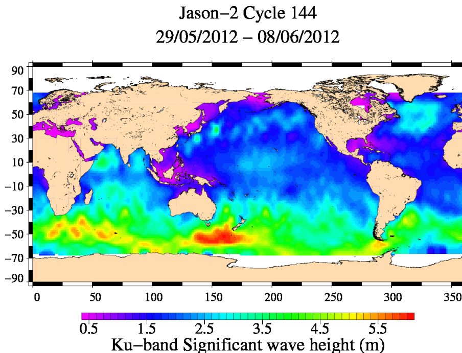
FIG. 5 – Significant wave height for cycle 144.
