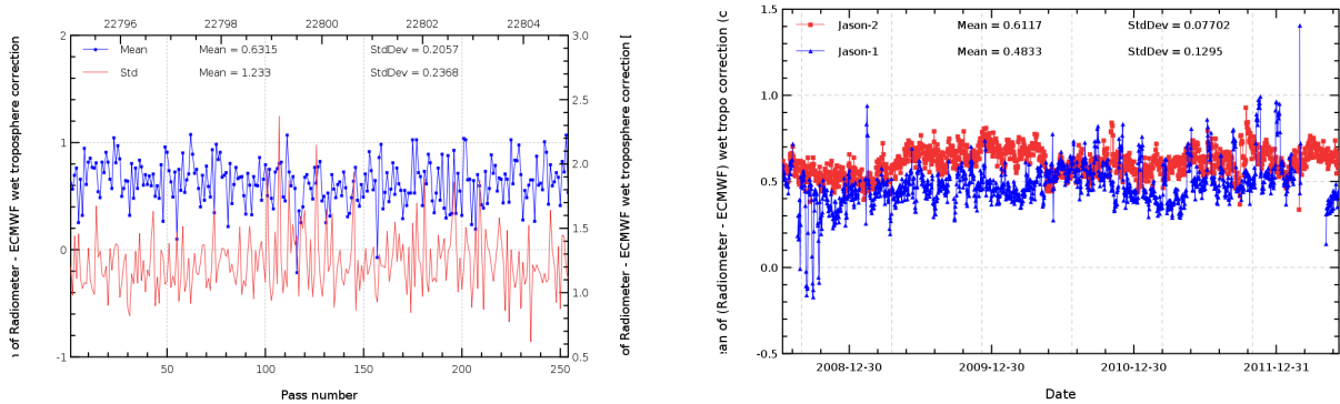
FIG. 11 – Pass monitoring of wet troposphere differences between radiometer and ECMWF model for Jason-2 cycle 144. (left) and Daily monitoring of wet troposphere differences between radiometer and ECMWF model (right).
