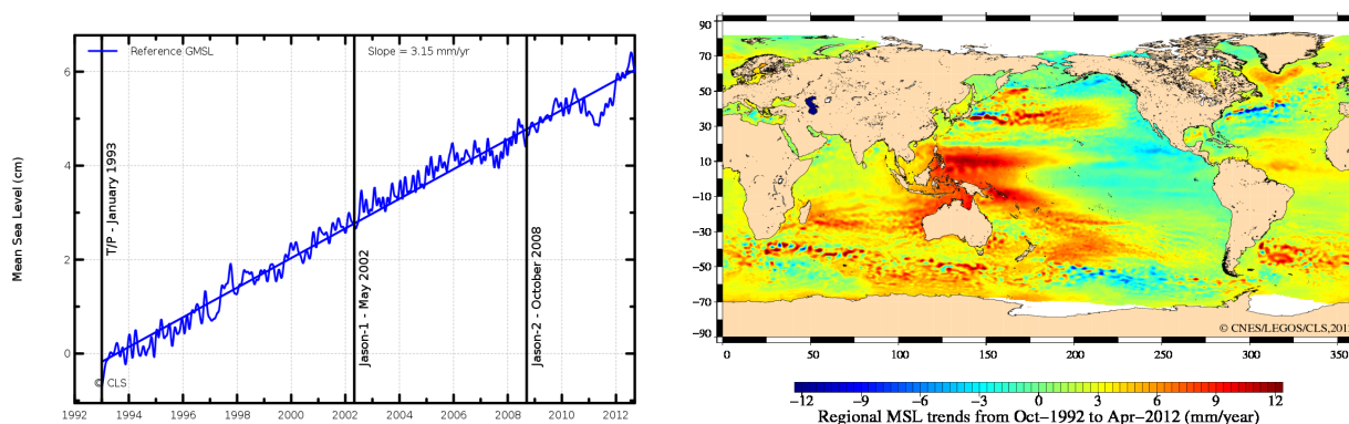
FIG. 21 – Global (left) and regional (right) MSL trends from 1993 onwards.
