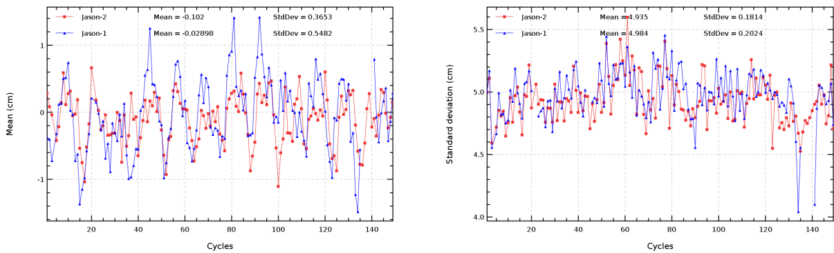
FIG. 13 – Cyclic monitoring of mean (left) and standard deviation (right) of SSH differences at crossovers for Jason-1 and Jason-2.
