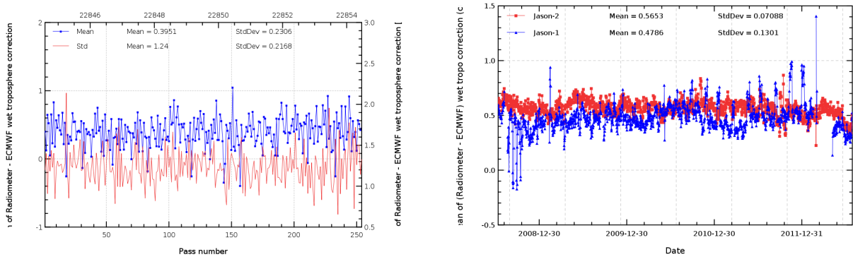
FIG. 11 – Pass monitoring of wet troposphere differences between radiometer and ECMWF model for Jason-2 cycle 149 (left) and daily monitoring of wet troposphere differences between radiometer and ECMWF model (right).
