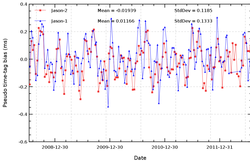
FIG. 15 – Cyclic monitoring of pseudo time tag bias for Jason-1 and Jason-2.
