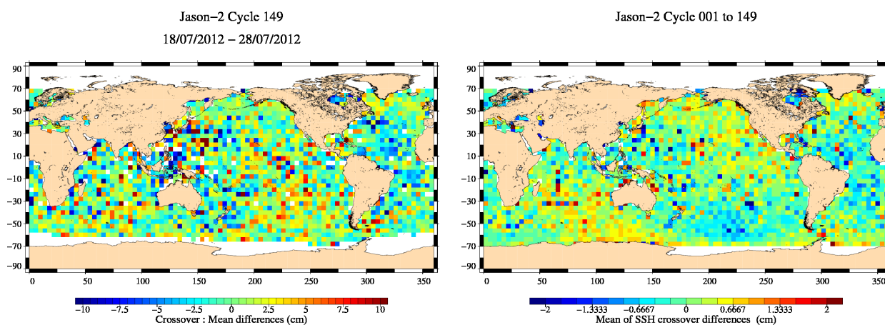
FIG. 12 – Mean SSH at crossovers for cycle 149 (left) and over the whole Jason-2 period (right).
