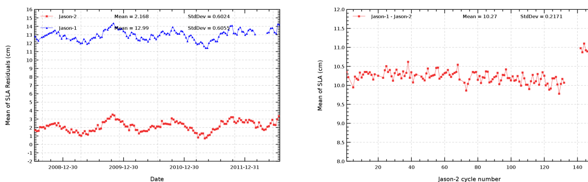
FIG. 16 – Cyclic monitoring of mean SLA for Jason-1 and Jason-2 (left) and differences of (Jason-1 – Jason-2) mean SLA (right).
