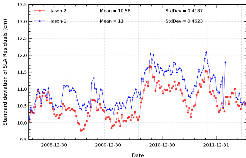
FIG. 20 – Cyclic monitoring standard deviation of along track SLA for Jason-1 and Jason-2.
