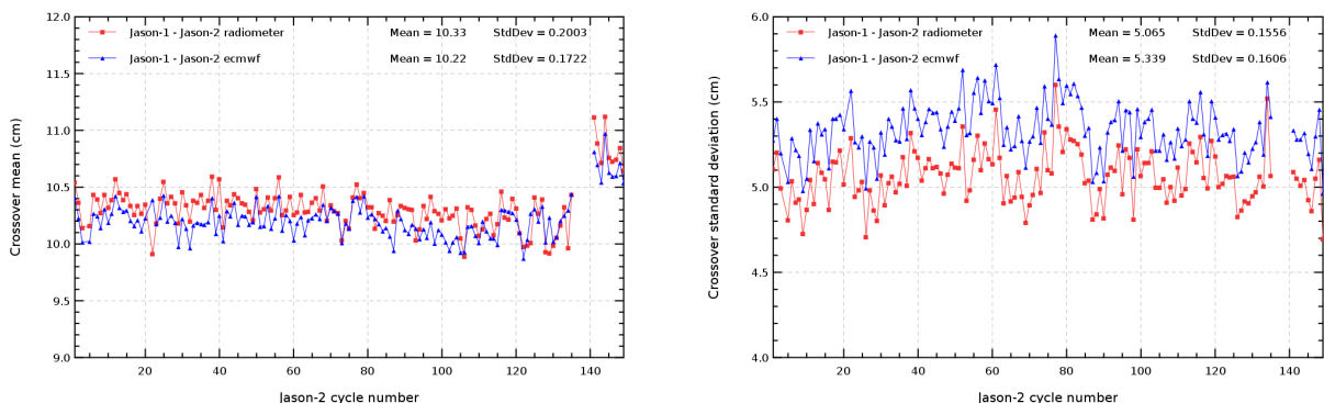
FIG. 14 – Cyclic monitoring of mean (left) and standard deviation (right) of (Jason-1 – Jason-2) SSH differences at crossovers.
