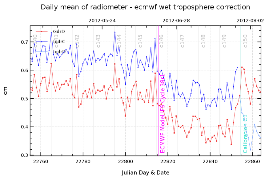
FIG. 12 – Daily monitoring of wet troposphere differences between radiometer and ECMWF model for Jason-2 cycles 140 to 150 in Gdr and Igdr.
