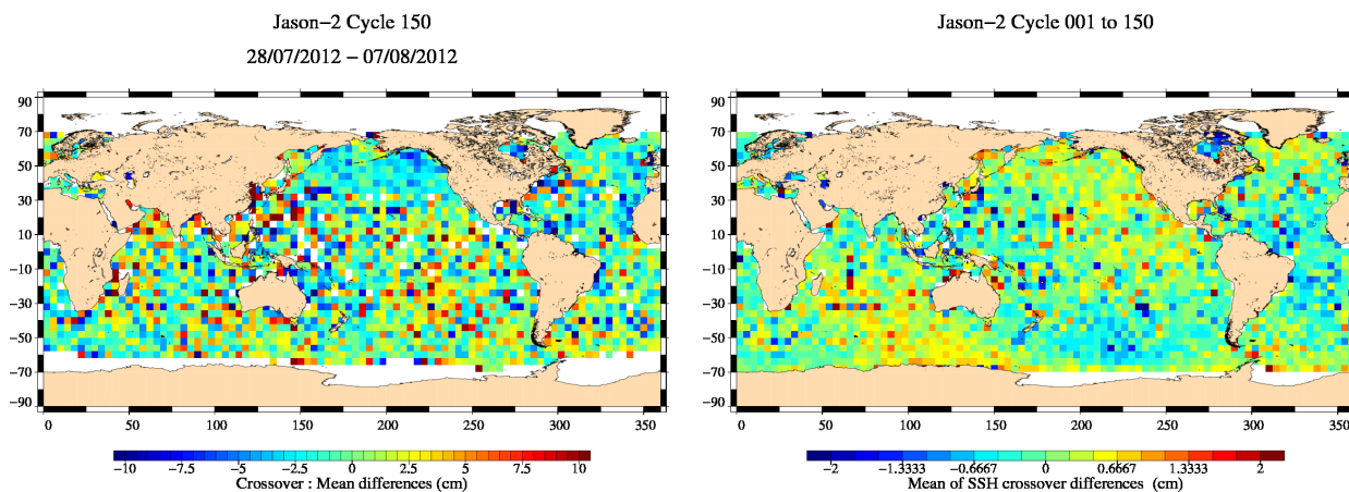
FIG. 13 – Mean SSH at crossovers for cycle 150 (left) and over the whole Jason-2 period (right).
