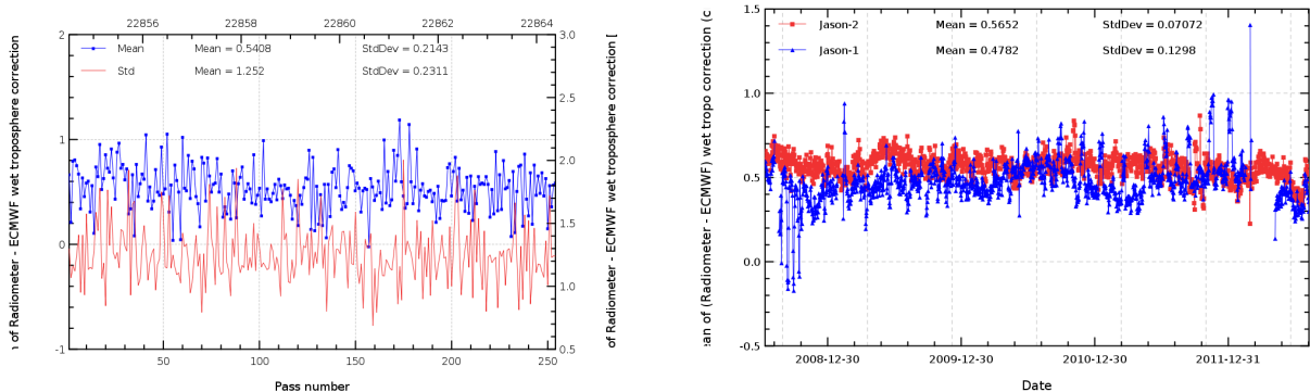
FIG. 11 – Pass monitoring of wet troposphere differences between radiometer and ECMWF model for Jason-2 cycle 150 (left) and daily monitoring of wet troposphere differences between radiometer and ECMWF model (right).
