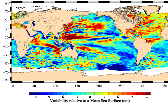
FIG. 17 – Sea level anomaly relative to MSS for cycle 152.
