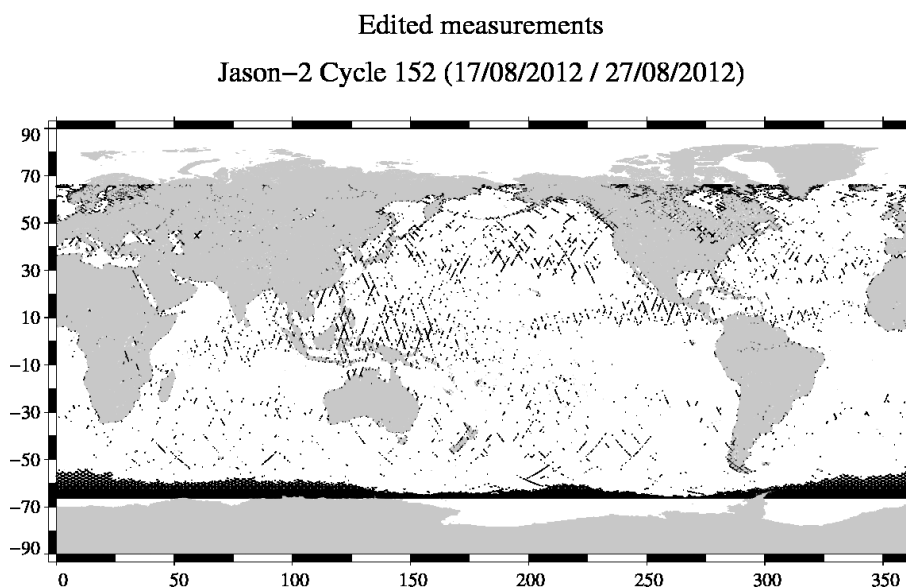
FIG. 2 – Edited measurements for cycle 152.
