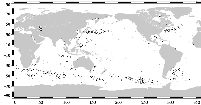
FIG. 18 – Differences higher than a 30 cm threshold for cycle 152.
