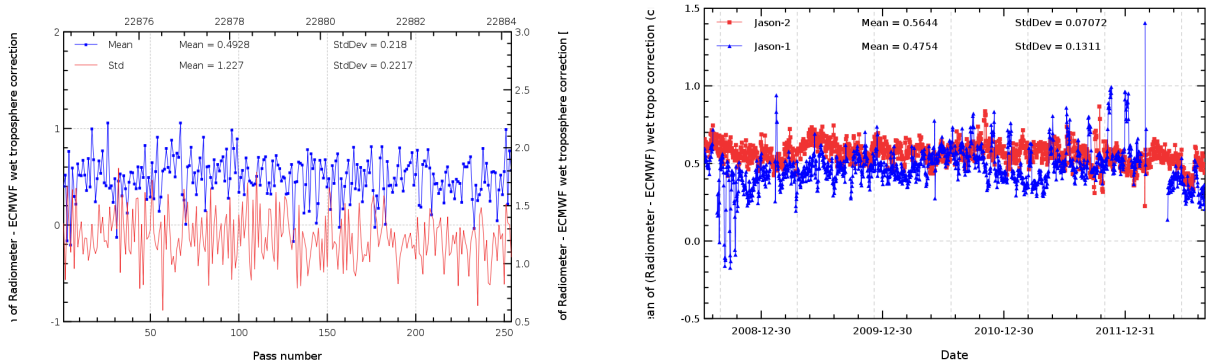
FIG. 11 – Pass monitoring of wet troposphere differences between radiometer and ECMWF model for Jason-2 cycle 152 (left) and daily monitoring of wet troposphere differences between radiometer and ECMWF model (right).
