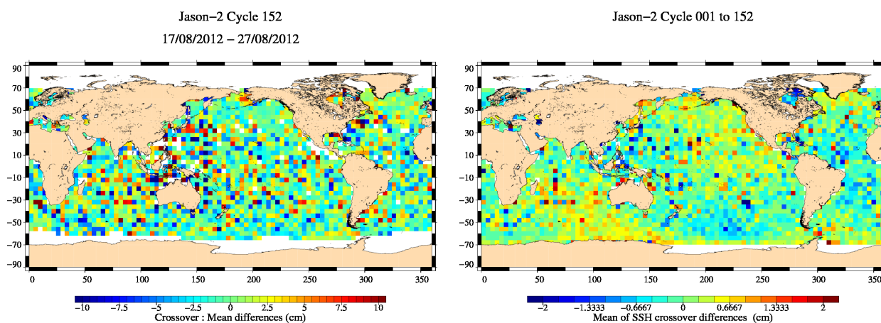
FIG. 12 – Mean SSH at crossovers for cycle 152 (left) and over the whole Jason-2 period (right).
