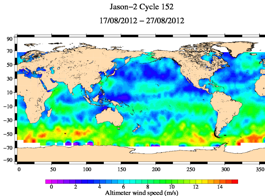
FIG. 9 – Altimeter wind speed for cycle 152.
