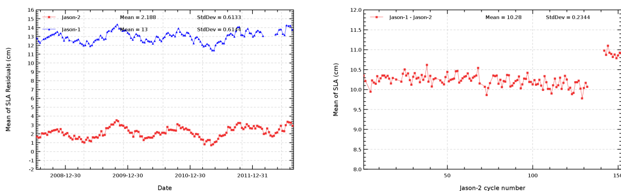
FIG. 16 – Cyclic monitoring of mean SLA for Jason-1 and Jason-2 (left) and differences of (Jason-1 – Jason-2) mean SLA (right).
