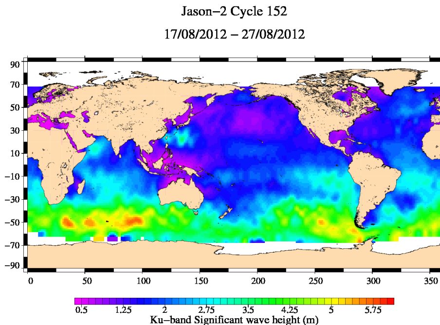
FIG. 5 – Significant wave height for cycle 152.
