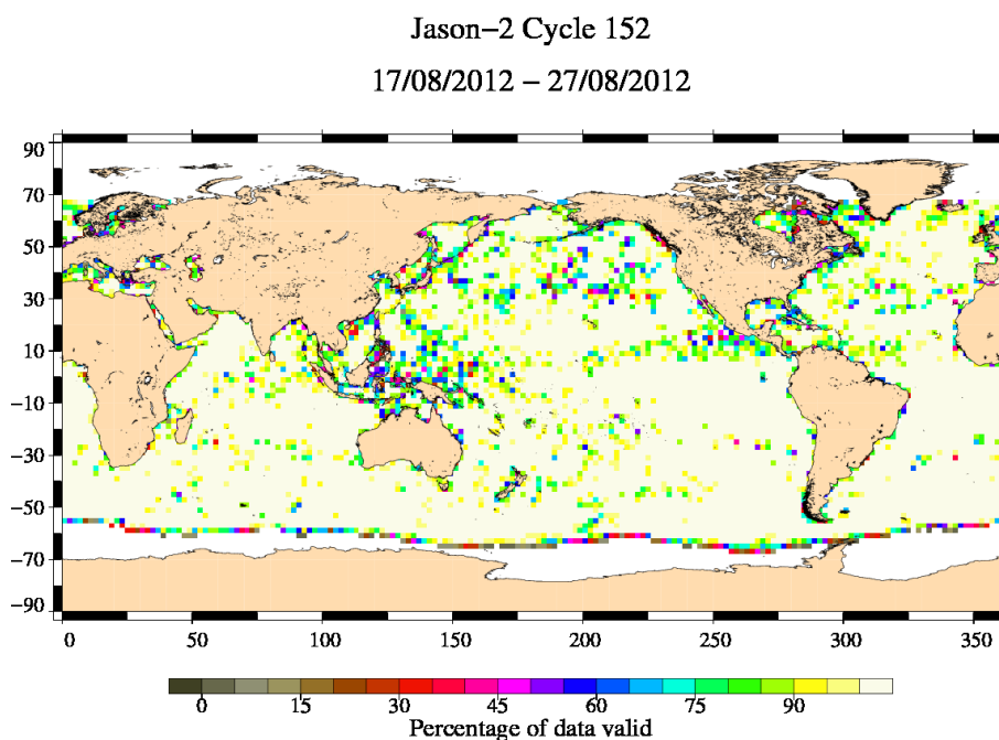
FIG. 3 – Percentage of valid measurements for cycle 152.
