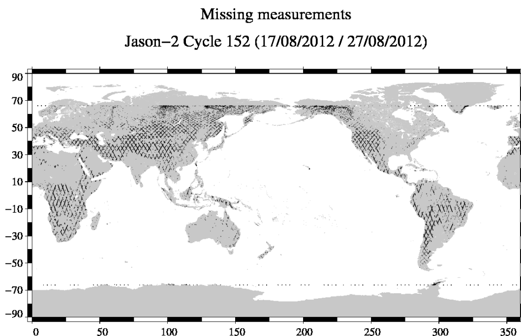
FIG. 1 – Missing measurements for cycle 152.
