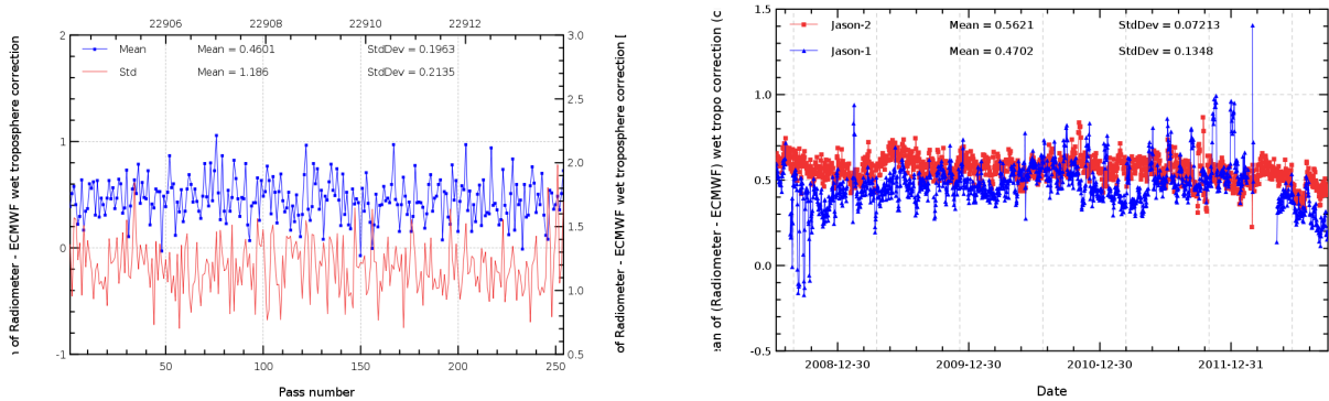
FIG. 11 – Pass monitoring of wet troposphere differences between radiometer and ECMWF model for Jason-2 cycle 155 (left) and daily monitoring of wet troposphere differences between radiometer and ECMWF model (right).
