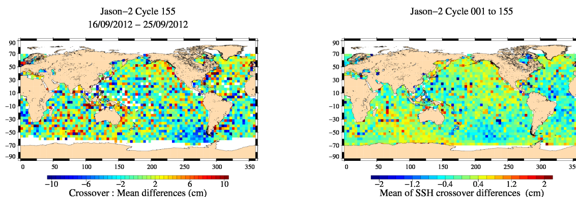
FIG. 12 – Mean SSH at crossovers for cycle 155 (left) and over the whole Jason-2 period (right).
