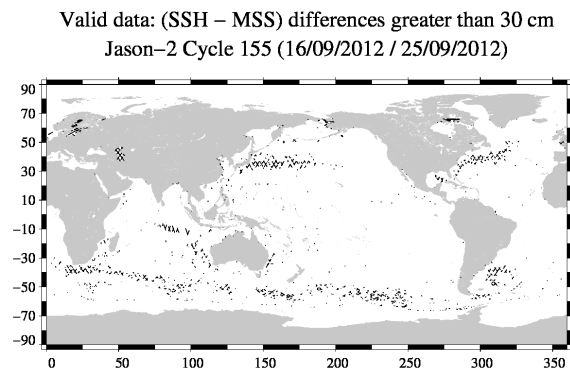
FIG. 17 – Sea level anomaly relative to MSS for cycle 155.
