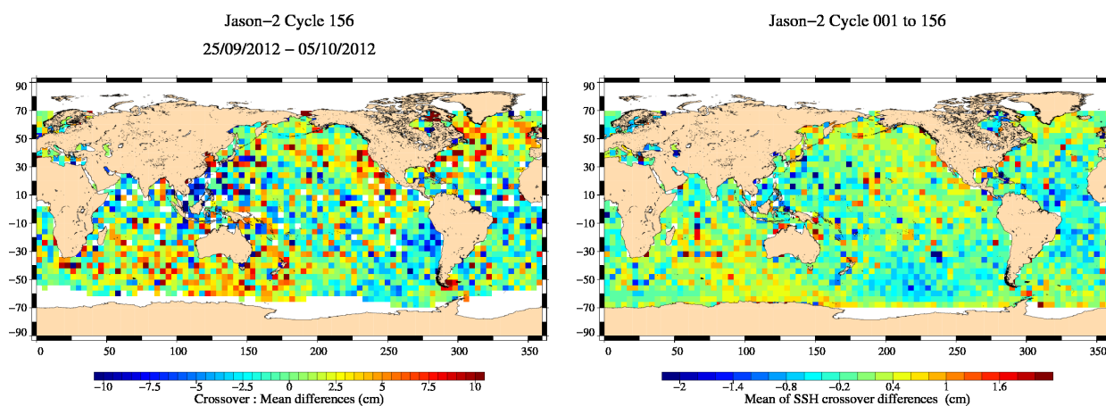
FIG. 13 – Mean SSH at crossovers for cycle 156 (left) and over the whole Jason-2 period (right).
