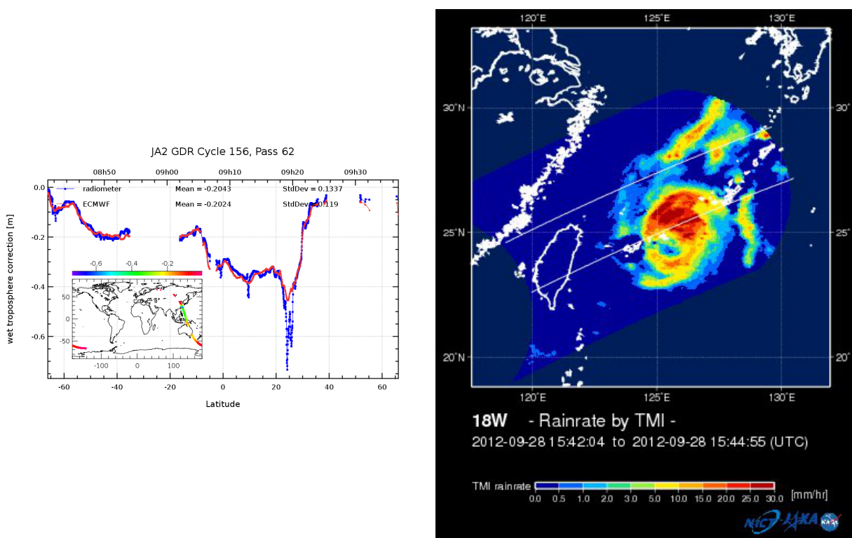
FIG. 3 – Left : Along-track radiometer and ECMWF model wet troposphere correction for pass 062. Right : Rain rates from TMI (from http://sharaku.eorc.jaxa.jp/TYPHOON_RT/data/trmm/asia/1218W/r2A12.51575.1218W.1.jpg )
