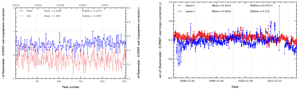
FIG. 12 – Pass monitoring of wet troposphere differences between radiometer and ECMWF model for Jason-2 cycle 156 (left) and daily monitoring of wet troposphere differences between radiometer and ECMWF model (right).
