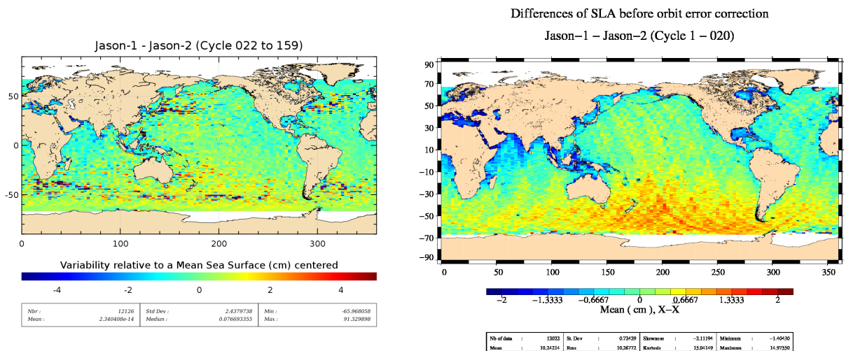
FIG. 19 – Jason-1 – Jason-2 SLA differences averaged over whole Jason-2 period since cycle 022 (left), and for flight formation phase (cycle 001 to 020) (right).
