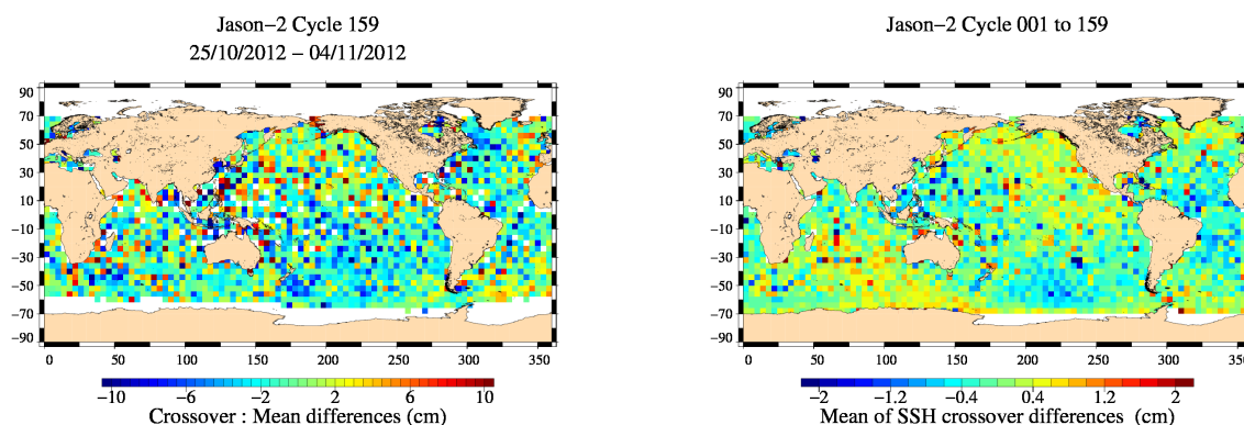
FIG. 12 – Mean SSH at crossovers for cycle 159 (left) and over the whole Jason-2 period (right).
