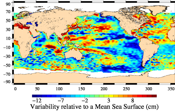
Jason-2 Cycle 159 25/10/2012 – 04/11/2012
