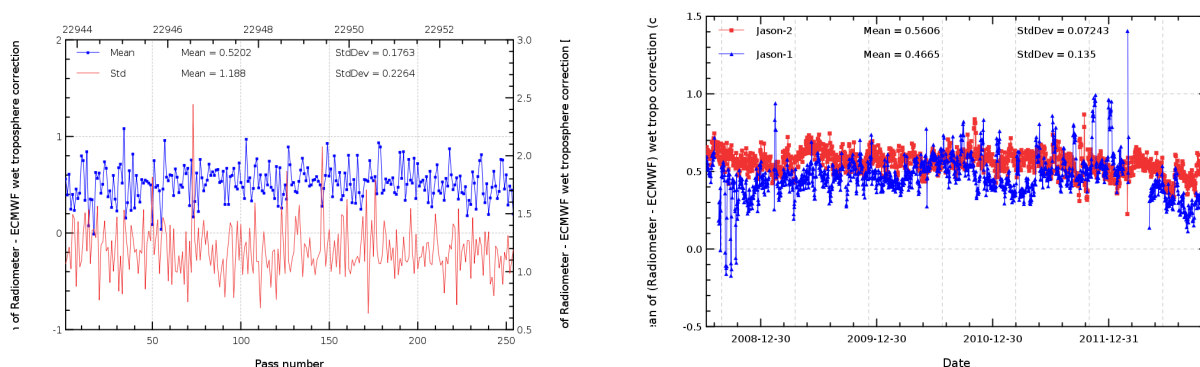
FIG. 11 – Pass monitoring of wet troposphere differences between radiometer and ECMWF model for Jason-2 cycle 159 (left) and daily monitoring of wet troposphere differences between radiometer and ECMWF model (right).
