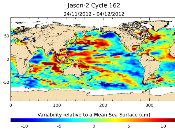
FIGURE 17 – Sea level anomaly relative to MSS for cycle 162.
