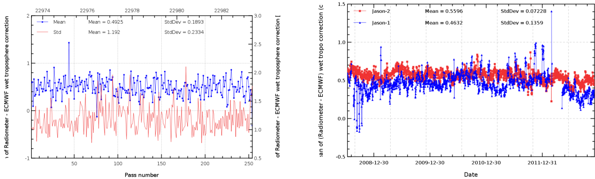
FIGURE 11 – Pass monitoring of wet troposphere differences between radiometer and ECMWF model for Jason-2 cycle 162 (left) and daily monitoring of wet troposphere differences between radiometer and ECMWF model (right).
