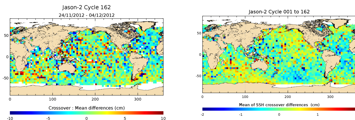
FIGURE 12 – Mean SSH at crossovers for cycle 162 (left) and over the whole Jason-2 period (right).
