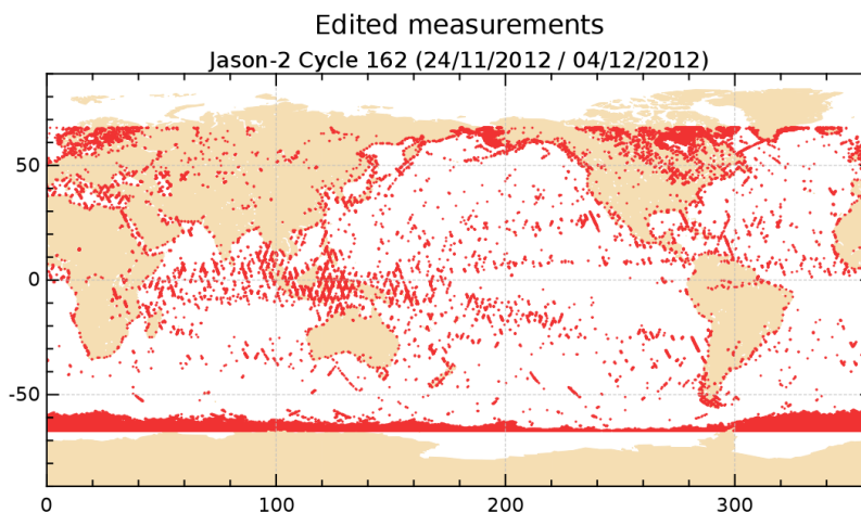
FIGURE 2 – Edited measurements for cycle 162.
