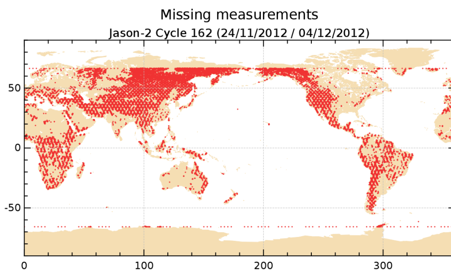
FIGURE 1 – Missing measurements for cycle 162.
