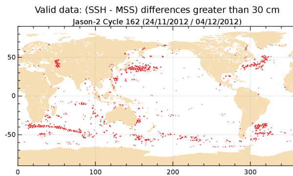
FIGURE 18 – Differences higher than a 30 cm threshold for cycle 162.
