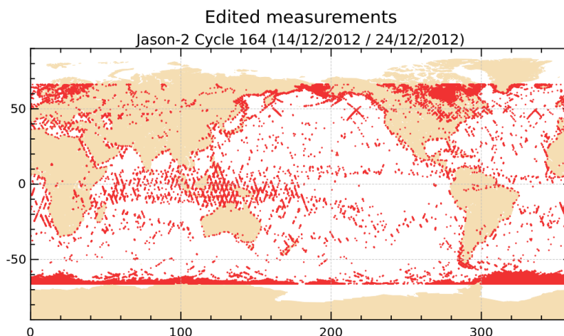
FIGURE 2 – Edited measurements for cycle 164.
