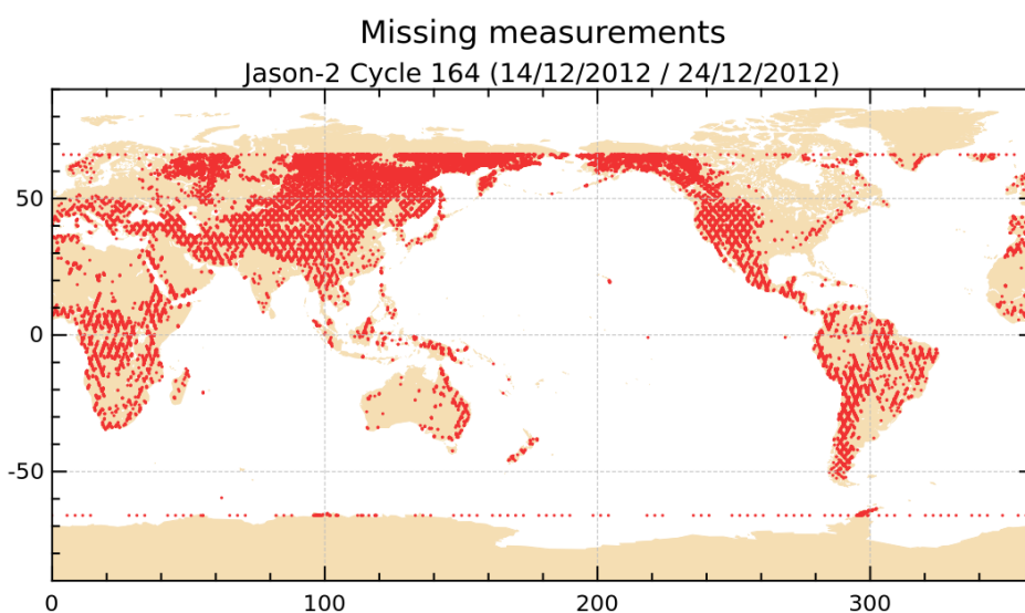
FIGURE 1 – Missing measurements for cycle 164.
