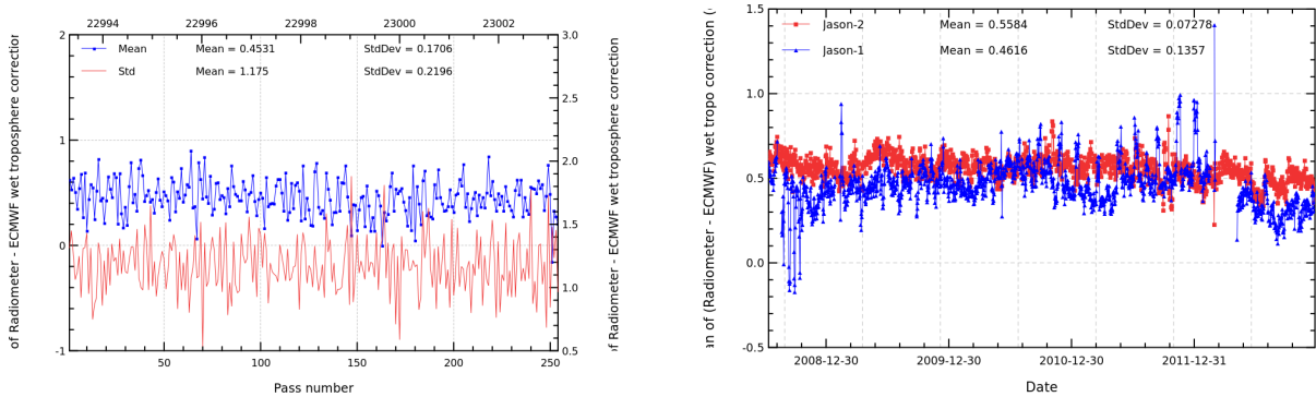
FIGURE 12 – Pass monitoring of wet troposphere differences between radiometer and ECMWF model for Jason-2 cycle 164 (left) and daily monitoring of wet troposphere differences between radiometer and ECMWF model (right).
