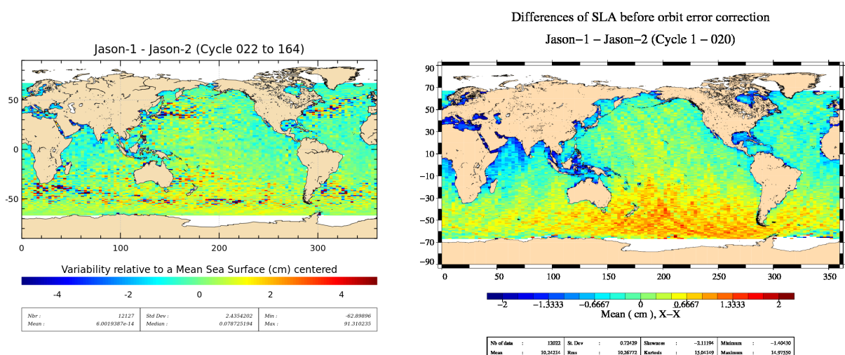
FIGURE 20 – Jason-1 – Jason-2 SLA differences averaged over whole Jason-2 period since cycle 022 (left), and for flight formation phase (cycle 001 to 020) (right).
