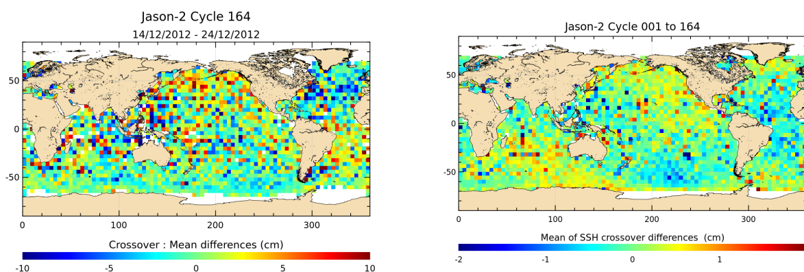
FIGURE 13 – Mean SSH at crossovers for cycle 164 (left) and over the whole Jason-2 period (right).
