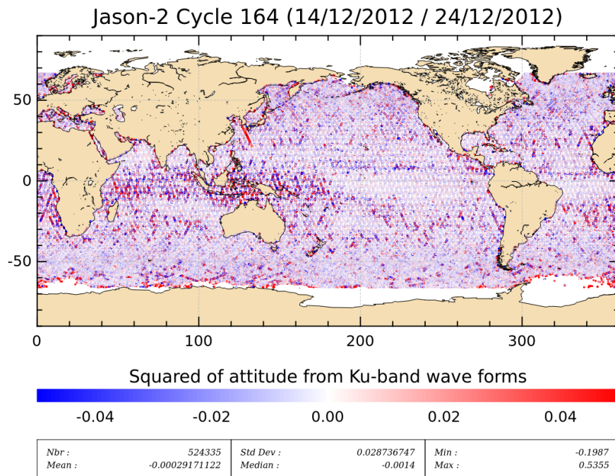
FIGURE 4 – Apparent squared mispointing from waveforms for cycle 164.
