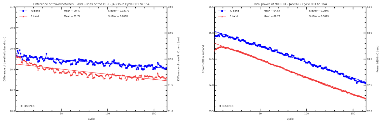
FIGURE 5 – Internal path delay (left) and total power of the PTR (right) for Ku- and C-band.
