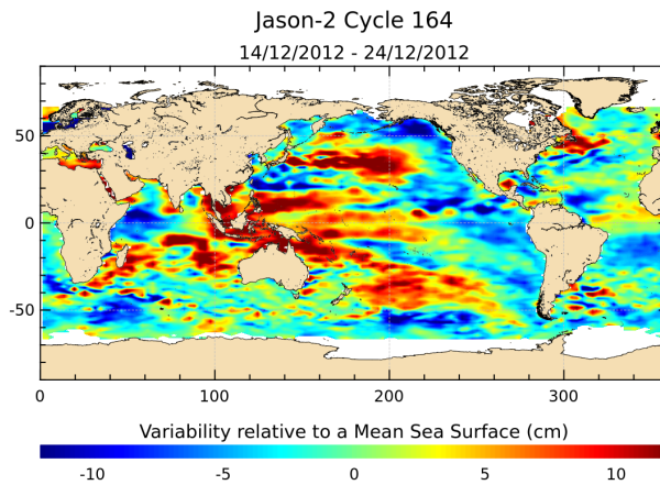
FIGURE 18 – Sea level anomaly relative to MSS for cycle 164.
