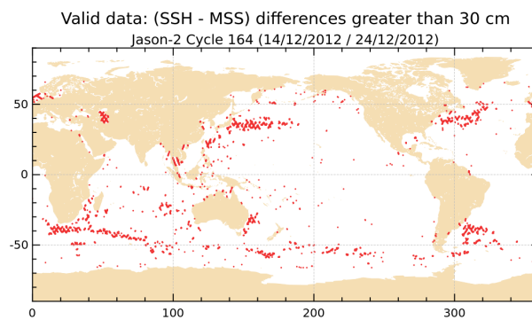
FIGURE 19 – Differences higher than a 30 cm threshold for cycle 164.
