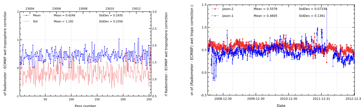
FIGURE 11 – Pass monitoring of wet troposphere differences between radiometer and ECMWF model for Jason-2 cycle 165 (left) and daily monitoring of wet troposphere differences between radiometer and ECMWF model (right).
