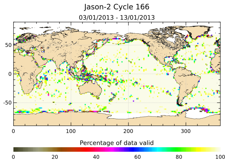
FIGURE 3 – Percentage of valid measurements for cycle 166.
