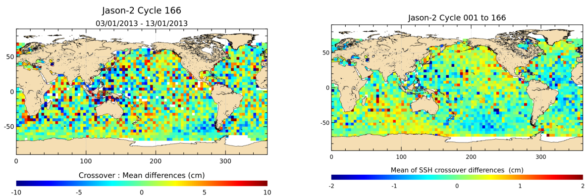
FIGURE 12 – Mean SSH at crossovers for cycle 166 (left) and over the whole Jason-2 period (right).
