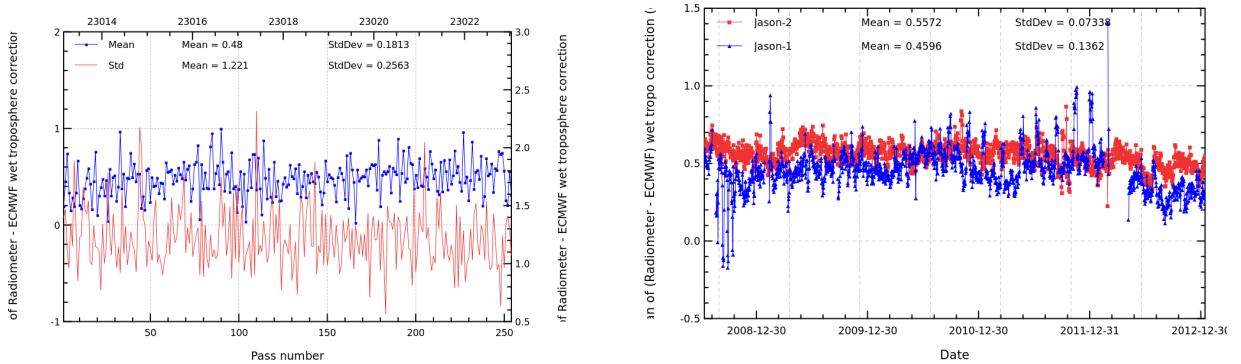
FIGURE 11 – Pass monitoring of wet troposphere differences between radiometer and ECMWF model for Jason-2 cycle 166 (left) and daily monitoring of wet troposphere differences between radiometer and ECMWF model (right).
