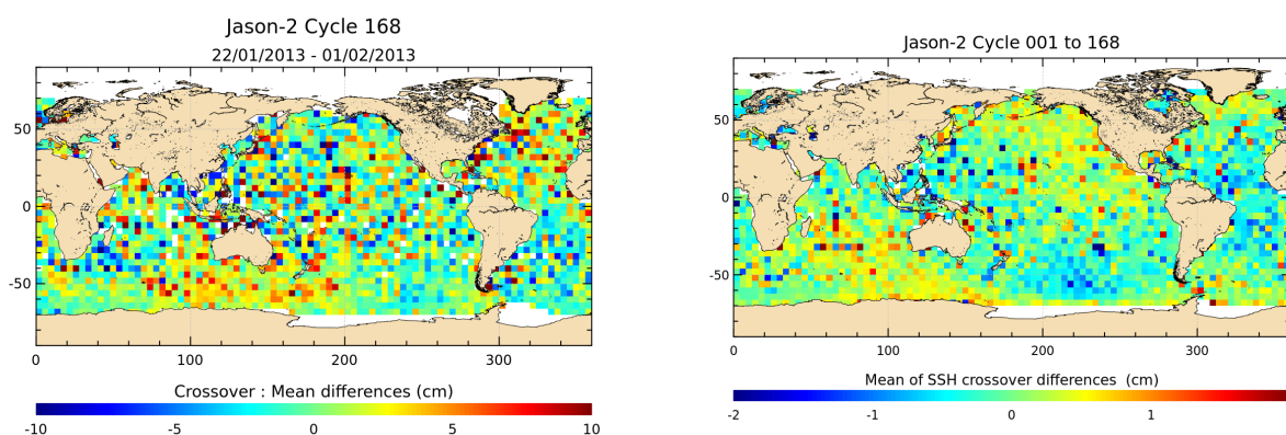
FIG. 12 – Mean SSH at crossovers for cycle 168 (left) and over the whole Jason-2 period (right).
