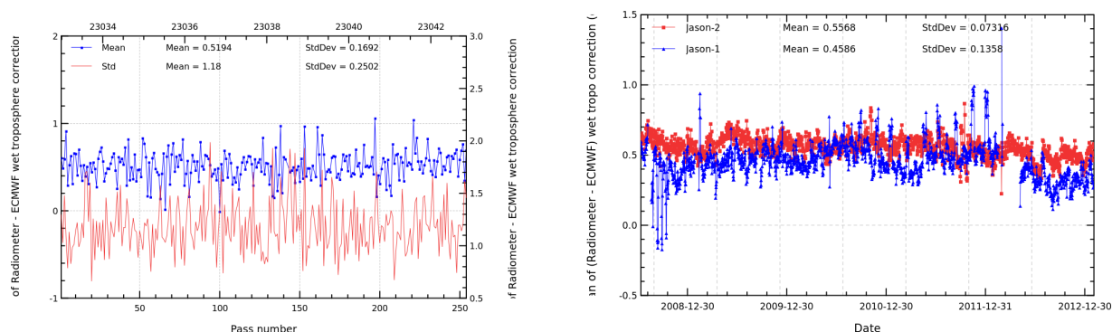
FIG. 11 – Pass monitoring of wet troposphere differences between radiometer and ECMWF model for Jason-2 cycle 168 (left) and daily monitoring of wet troposphere differences between radiometer and ECMWF model (right).
