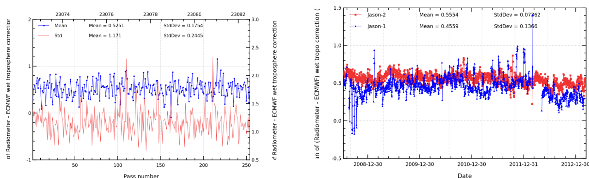
FIG. 11 – Pass monitoring of wet troposphere differences between radiometer and ECMWF model for Jason-2 cycle 172 (left) and daily monitoring of wet troposphere differences between radiometer and ECMWF model (right).
