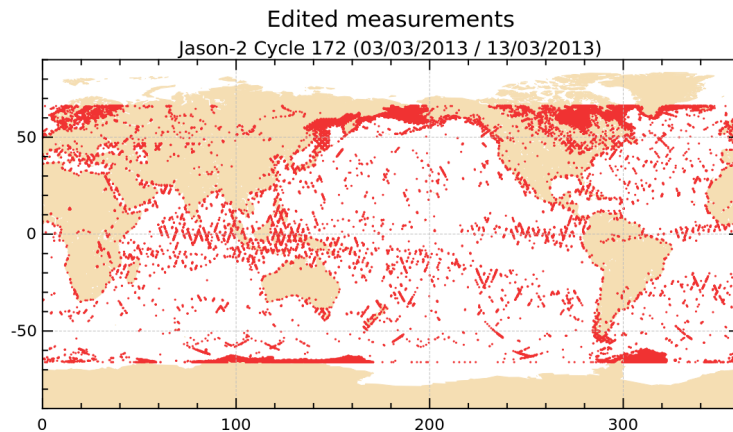
FIG. 2 – Edited measurements for cycle 172.
