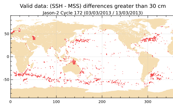
FIG. 18 – Differences higher than a 30 cm threshold for cycle 172.
