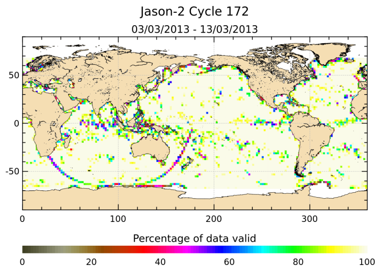
FIG. 3 – Percentage of valid measurements for cycle 172.
