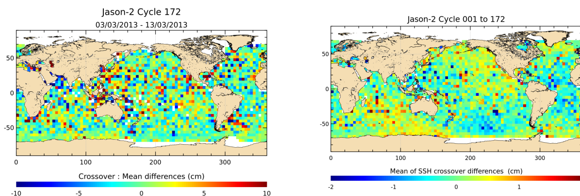
FIG. 12 – Mean SSH at crossovers for cycle 172 (left) and over the whole Jason-2 period (right).
