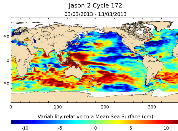
FIG. 17 – Sea level anomaly relative to MSS for cycle 172.
