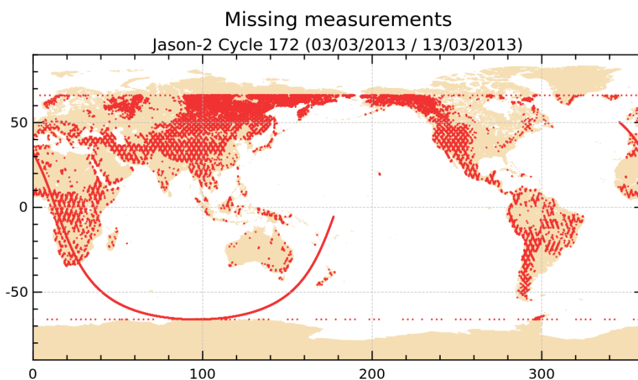
FIG. 1 – Missing measurements for cycle 172.
