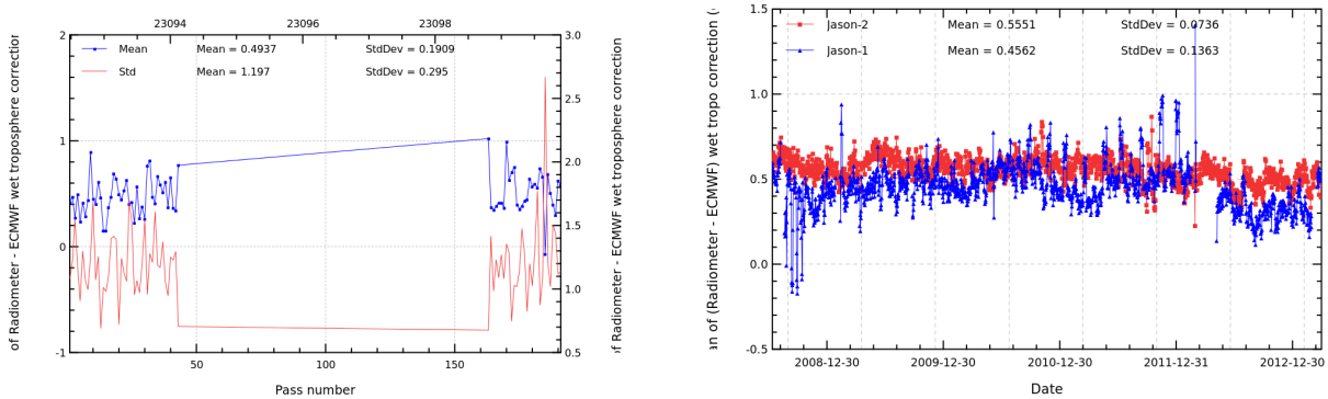
FIGURE 11 – Pass monitoring of wet troposphere differences between radiometer and ECMWF model for Jason-2 cycle 174 (left) and daily monitoring of wet troposphere differences between radiometer and ECMWF model (right).
