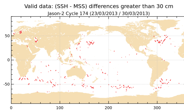
FIGURE 18 – Differences higher than a 30 cm threshold for cycle 174.
