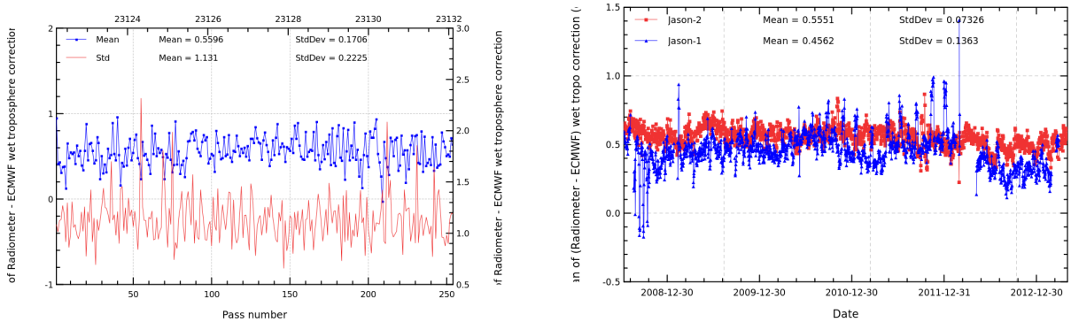
FIGURE 11 – Pass monitoring of wet troposphere differences between radiometer and ECMWF model for Jason-2 cycle 177 (left) and daily monitoring of wet troposphere differences between radiometer and ECMWF model (right).
