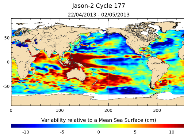
FIGURE 17 – Sea level anomaly relative to MSS for cycle 177.
