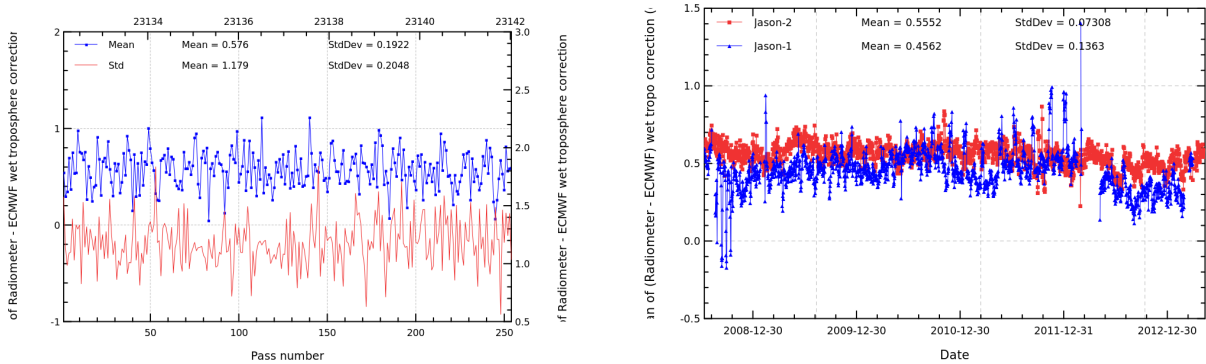
FIGURE 11 – Pass monitoring of wet troposphere differences between radiometer and ECMWF model for Jason-2 cycle 178 (left) and daily monitoring of wet troposphere differences between radiometer and ECMWF model (right).
