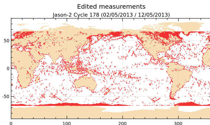
FIGURE 2 – Edited measurements for cycle 178.
