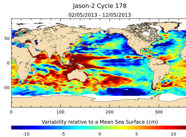
FIGURE 17 – Sea level anomaly relative to MSS for cycle 178.
