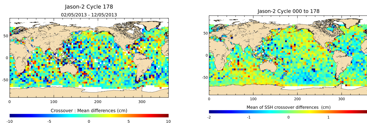
FIGURE 12 – Mean SSH at crossovers for cycle 178 (left) and over the whole Jason-2 period (right).
