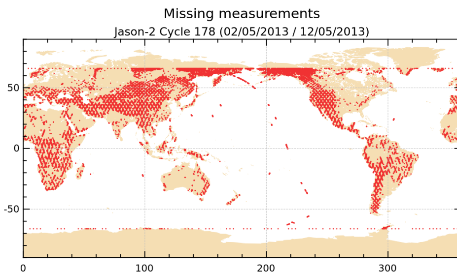
FIGURE 1 – Missing measurements for cycle 178.
