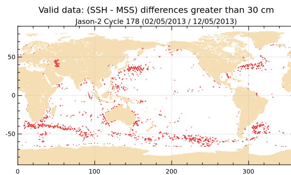
FIGURE 18 – Differences higher than a 30 cm threshold for cycle 178.
