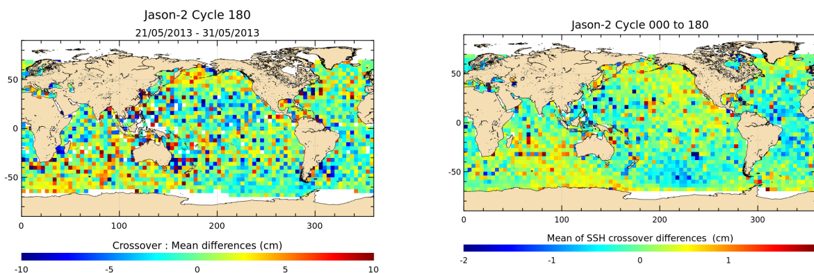
FIGURE 12 – Mean SSH at crossovers for cycle 180 (left) and over the whole Jason-2 period (right).
