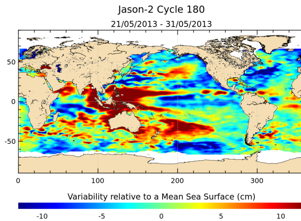
FIGURE 17 – Sea level anomaly relative to MSS for cycle 180.
