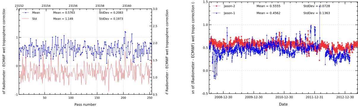
FIGURE 11 – Pass monitoring of wet troposphere differences between radiometer and ECMWF model for Jason-2 cycle 180 (left) and daily monitoring of wet troposphere differences between radiometer and ECMWF model (right).
