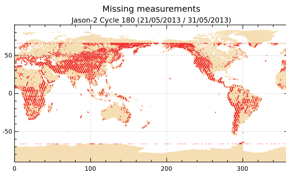
FIGURE 1 – Missing measurements for cycle 180.
