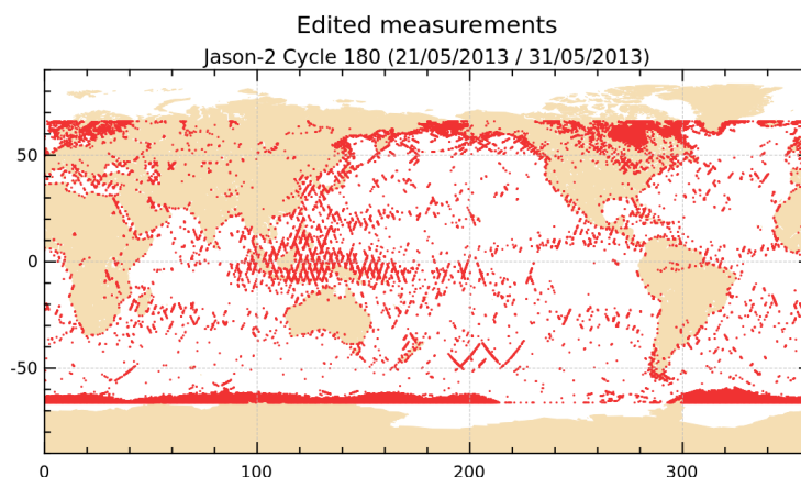
FIGURE 2 – Edited measurements for cycle 180.
