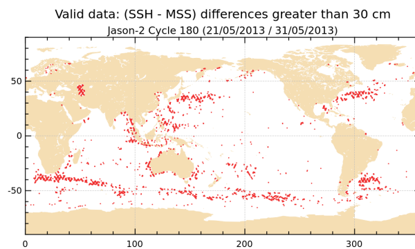
FIGURE 18 – Differences higher than a 30 cm threshold for cycle 180.
