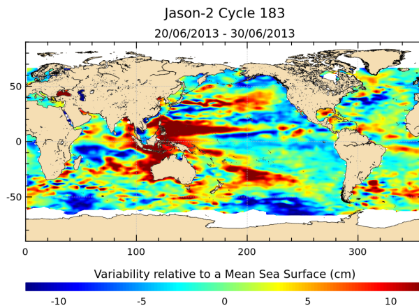
FIGURE 17 – Sea level anomaly relative to MSS for cycle 183.
