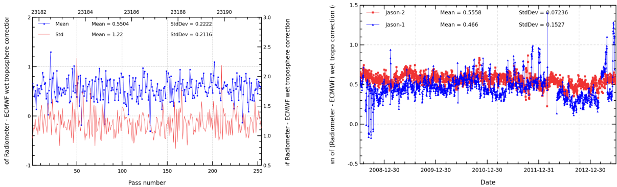
FIGURE 11 – Pass monitoring of wet troposphere differences between radiometer and ECMWF model for Jason-2 cycle 183 (left) and daily monitoring of wet troposphere differences between radiometer and ECMWF model (right).
