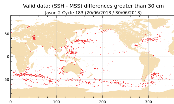
FIGURE 18 – Differences higher than a 30 cm threshold for cycle 183.
