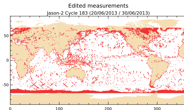
FIGURE 2 – Edited measurements for cycle 183.
