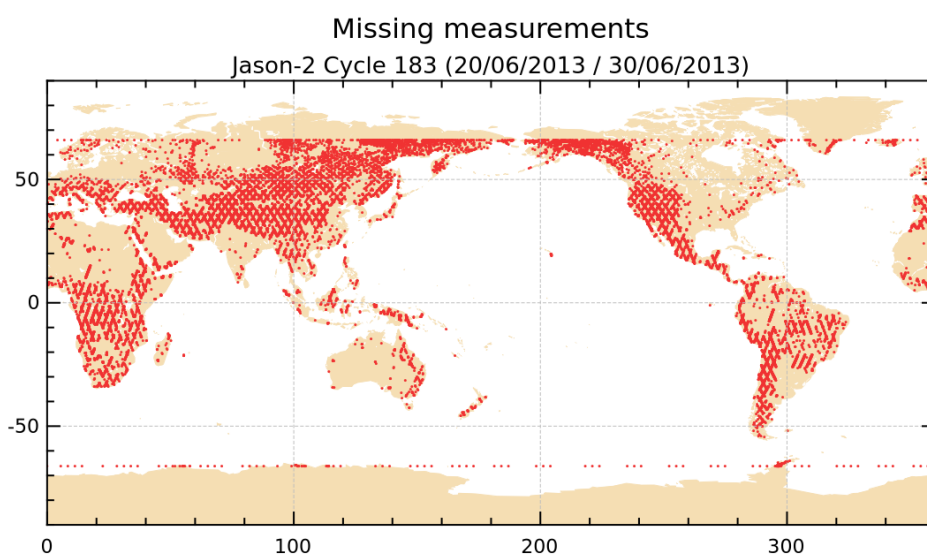
FIGURE 1 – Missing measurements for cycle 183.
