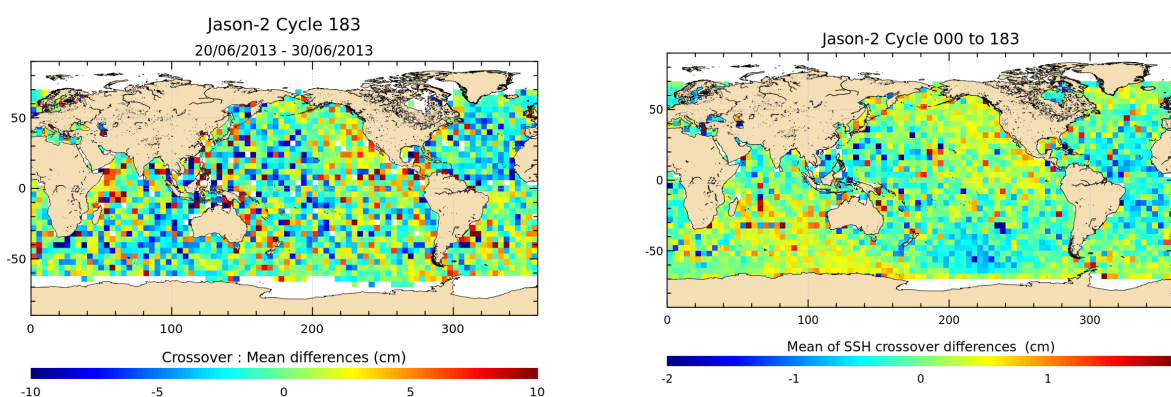
FIGURE 12 – Mean SSH at crossovers for cycle 183 (left) and over the whole Jason-2 period (right).
