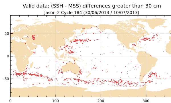
FIGURE 18 – Differences higher than a 30 cm threshold for cycle 184.
