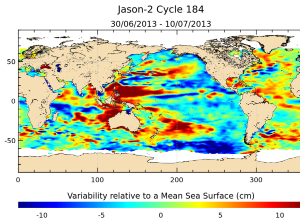
FIGURE 17 – Sea level anomaly relative to MSS for cycle 184.
