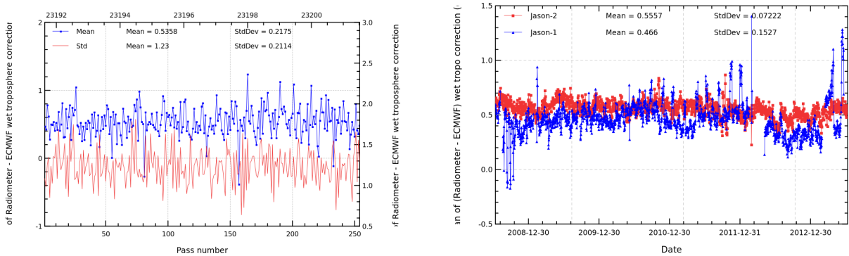
FIGURE 11 – Pass monitoring of wet troposphere differences between radiometer and ECMWF model for Jason-2 cycle 184 (left) and daily monitoring of wet troposphere differences between radiometer and ECMWF model (right).
