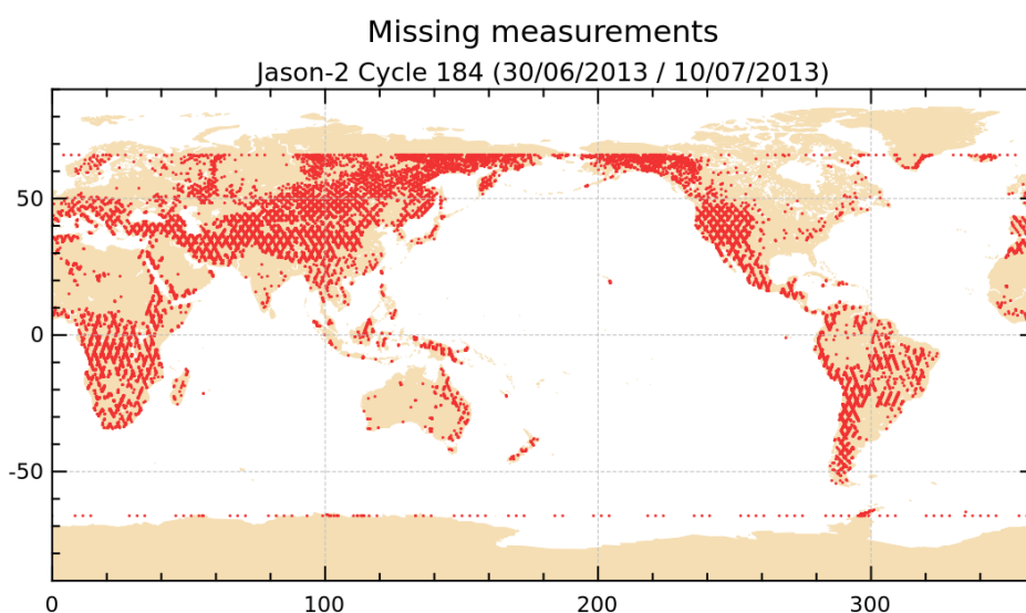
FIGURE 1 – Missing measurements for cycle 184.
