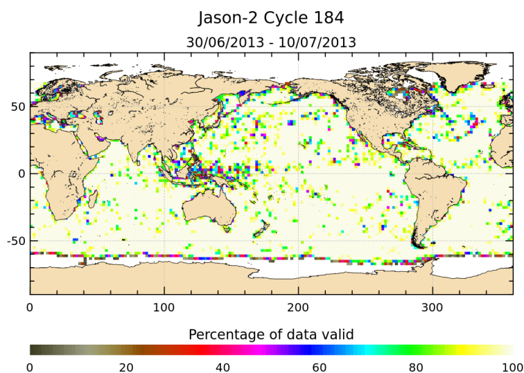
FIGURE 3 – Percentage of valid measurements for cycle 184.
