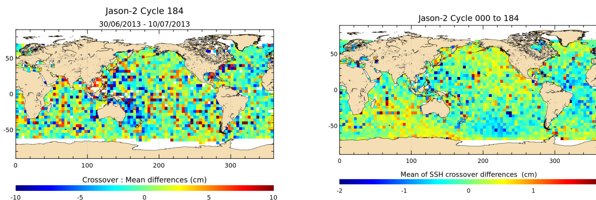
FIGURE 12 – Mean SSH at crossovers for cycle 184 (left) and over the whole Jason-2 period (right).
