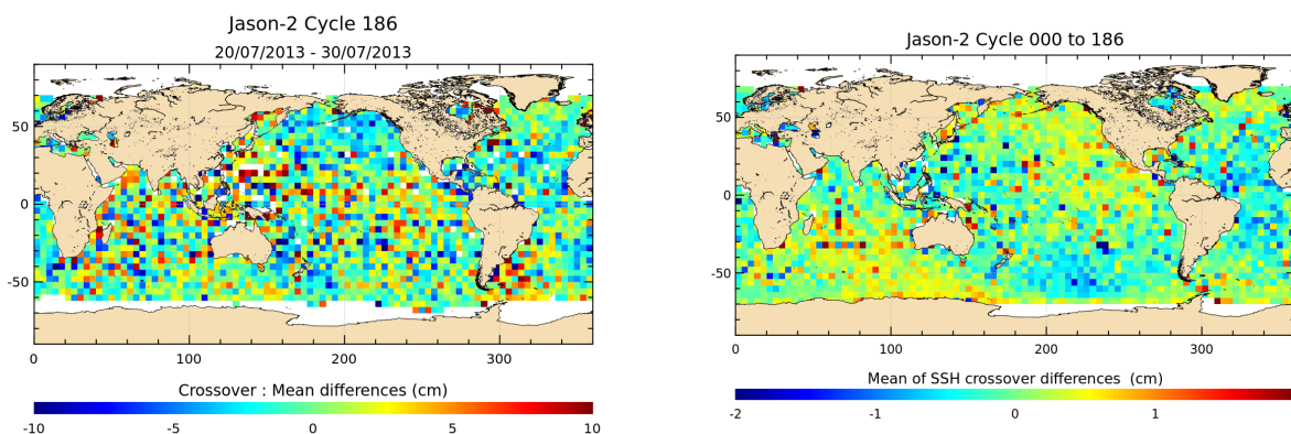
FIGURE 12 – Mean SSH at crossovers for cycle 186 (left) and over the whole Jason-2 period (right).
