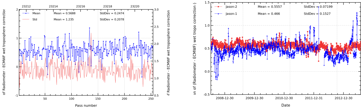
FIGURE 11 – Pass monitoring of wet troposphere differences between radiometer and ECMWF model for Jason-2 cycle 186 (left) and daily monitoring of wet troposphere differences between radiometer and ECMWF model (right).
