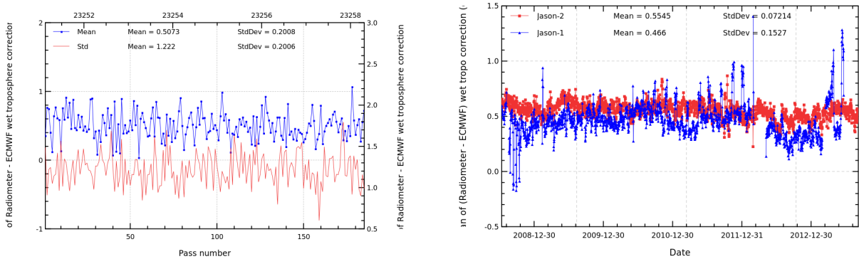
FIGURE 11 – Pass monitoring of wet troposphere differences between radiometer and ECMWF model for Jason-2 cycle 190 (left) and daily monitoring of wet troposphere differences between radiometer and ECMWF model (right).
