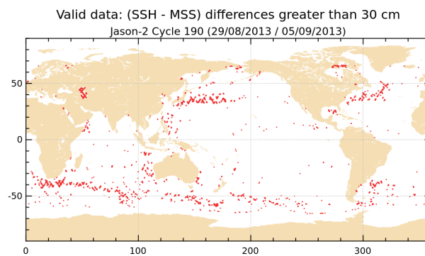
FIGURE 18 – Differences higher than a 30 cm threshold for cycle 190.
