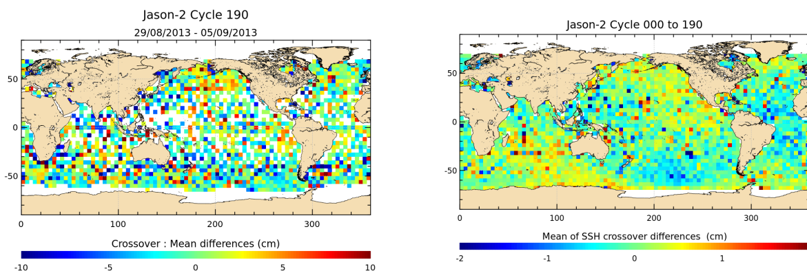
FIGURE 12 – Mean SSH at crossovers for cycle 190 (left) and over the whole Jason-2 period (right).
