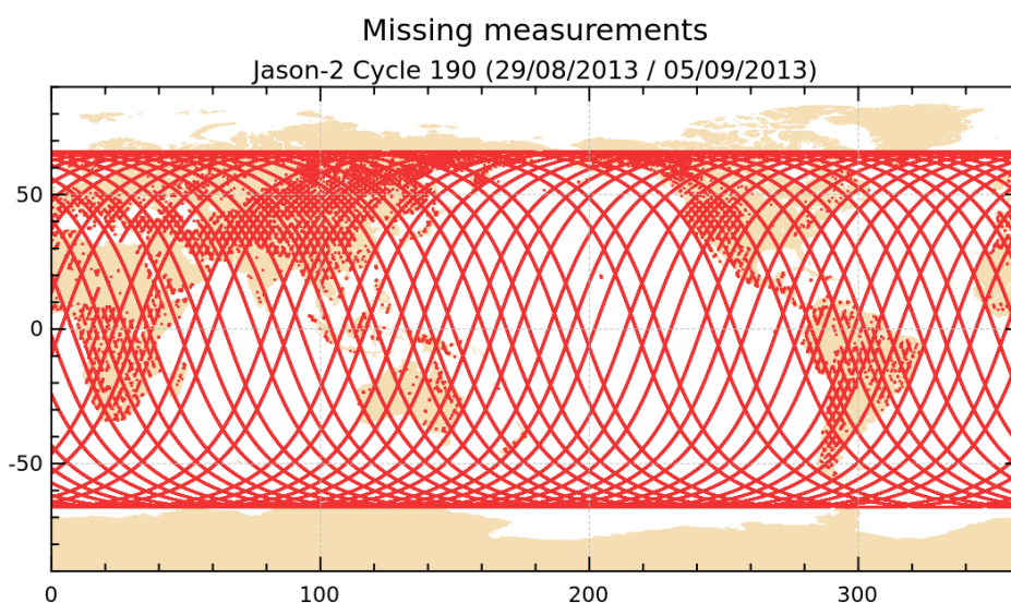
FIGURE 1 – Missing measurements for cycle 190.
