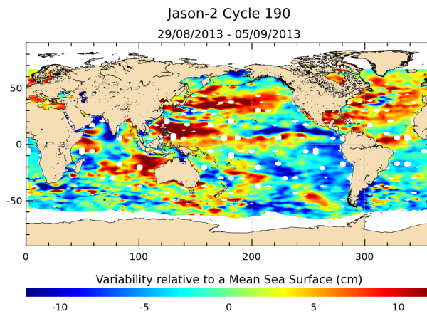
FIGURE 17 – Sea level anomaly relative to MSS for cycle 190.
