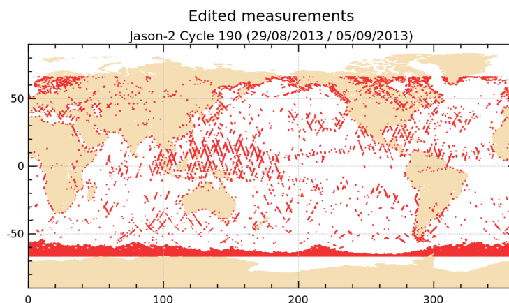
FIGURE 2 – Edited measurements for cycle 190.
