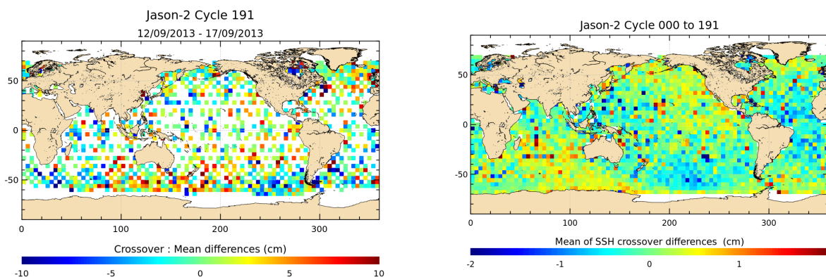
FIGURE 12 – Mean SSH at crossovers for cycle 191 (left) and over the whole Jason-2 period (right).
