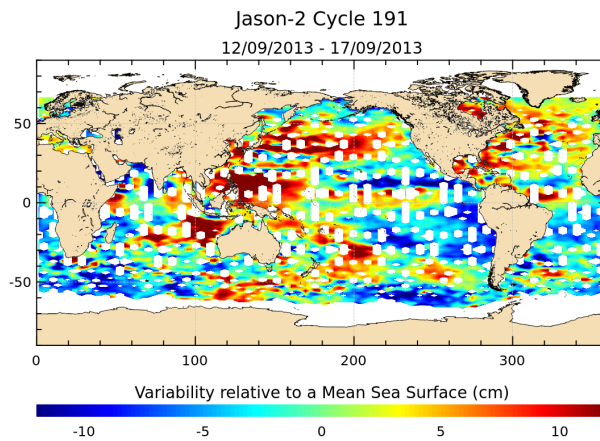
FIGURE 17 – Sea level anomaly relative to MSS for cycle 191.
