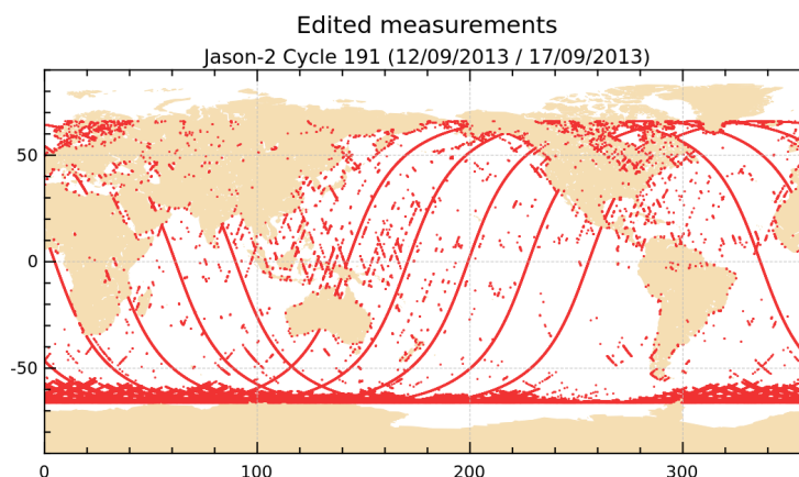
FIGURE 2 – Edited measurements for cycle 191.
