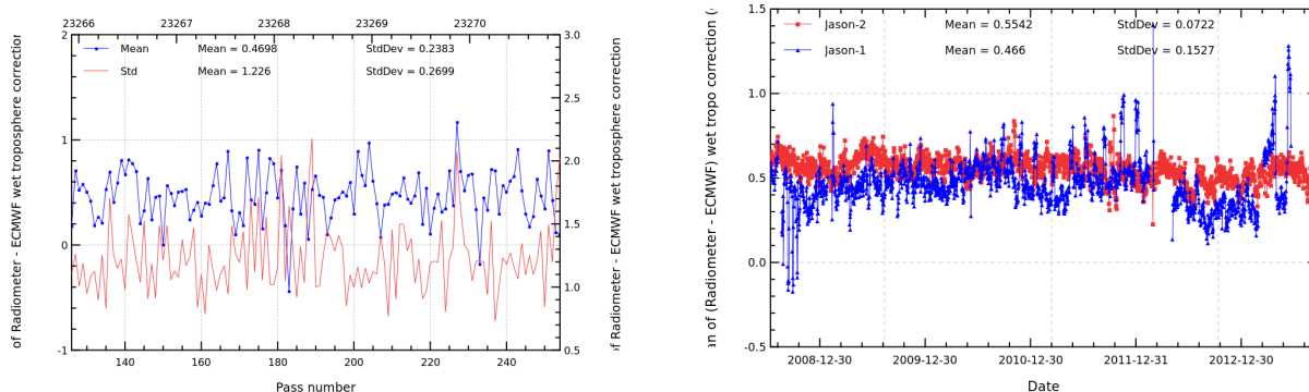
FIGURE 11 – Pass monitoring of wet troposphere differences between radiometer and ECMWF model for Jason-2 cycle 191 (left) and daily monitoring of wet troposphere differences between radiometer and ECMWF model (right).
