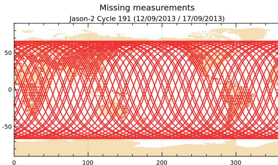
FIGURE 1 – Missing measurements for cycle 191.
