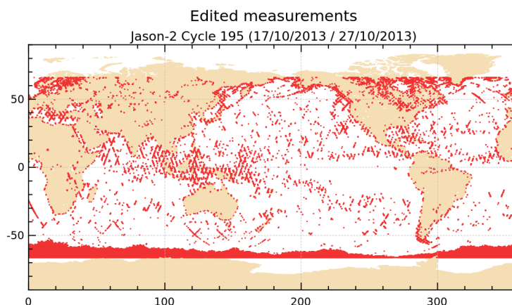
FIGURE 2 – Edited measurements for cycle 195.
