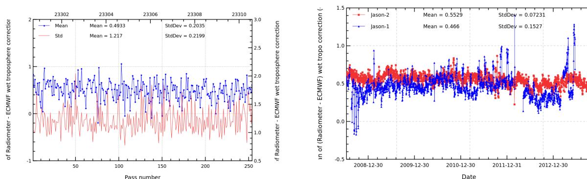
FIGURE 11 – Pass monitoring of wet troposphere differences between radiometer and ECMWF model for Jason-2 cycle 195 (left) and daily monitoring of wet troposphere differences between radiometer and ECMWF model (right).
