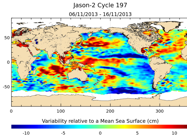
FIGURE 17 – Sea level anomaly relative to MSS for cycle 197.
