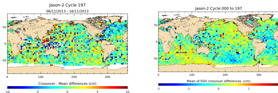
FIGURE 12 – Mean SSH at crossovers for cycle 197 (left) and over the whole Jason-2 period (right).
