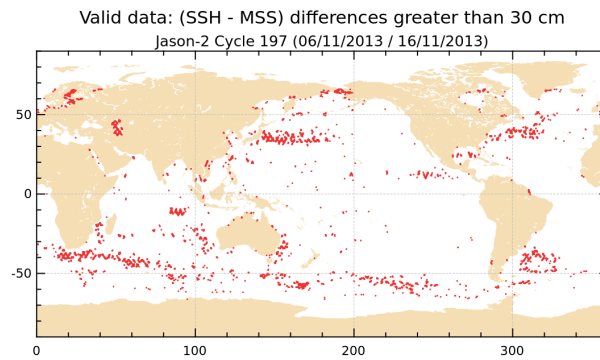
FIGURE 18 – Differences higher than a 30 cm threshold for cycle 197.
