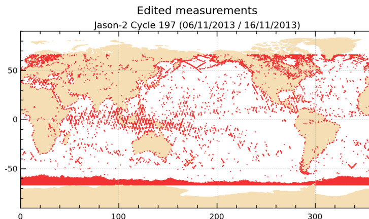
FIGURE 2 – Edited measurements for cycle 197.
