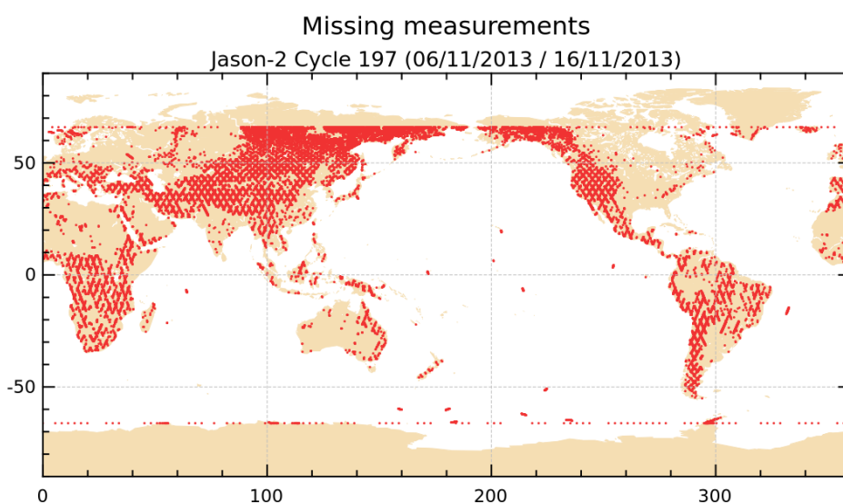
FIGURE 1 – Missing measurements for cycle 197.
