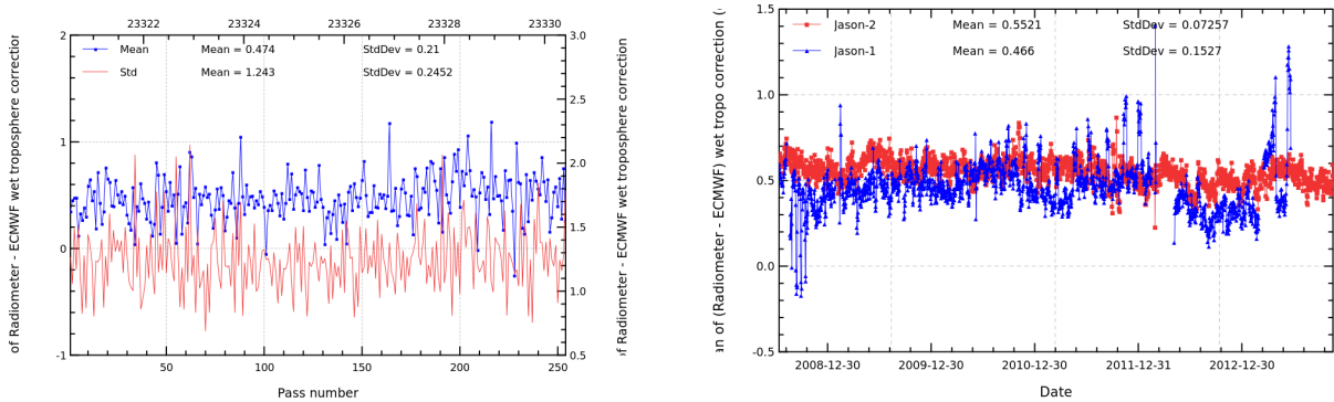
FIGURE 11 – Pass monitoring of wet troposphere differences between radiometer and ECMWF model for Jason-2 cycle 197 (left) and daily monitoring of wet troposphere differences between radiometer and ECMWF model (right).
