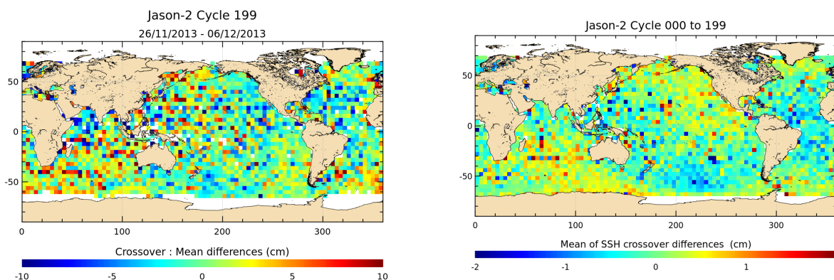
FIGURE 12 – Mean SSH at crossovers for cycle 199 (left) and over the whole Jason-2 period (right).
