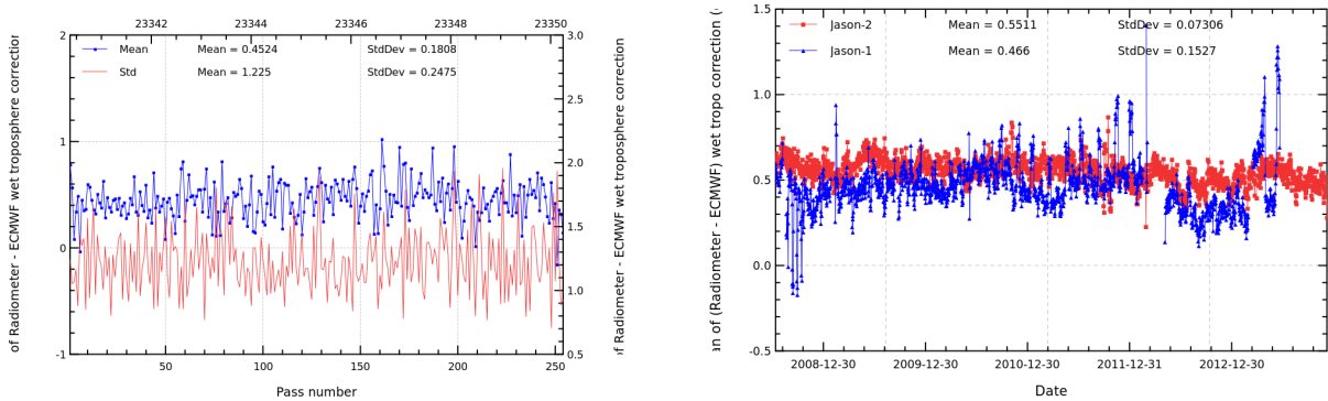
FIGURE 11 – Pass monitoring of wet troposphere differences between radiometer and ECMWF model for Jason-2 cycle 199 (left) and daily monitoring of wet troposphere differences between radiometer and ECMWF model (right).
