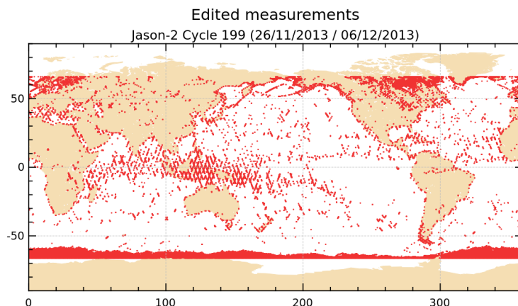
FIGURE 2 – Edited measurements for cycle 199.
