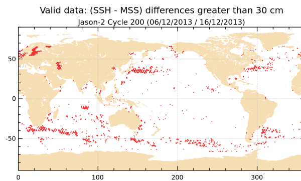
FIGURE 19 – Differences higher than a 30 cm threshold for cycle 200.
