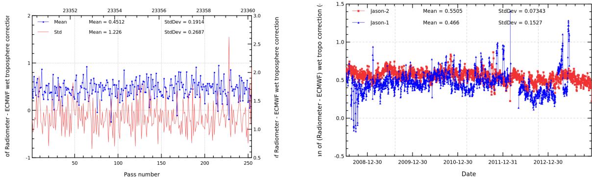
FIGURE 12 – Pass monitoring of wet troposphere differences between radiometer and ECMWF model for Jason-2 cycle 200 (left) and daily monitoring of wet troposphere differences between radiometer and ECMWF model (right).
