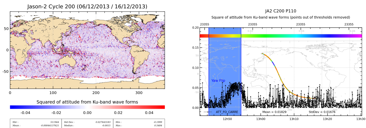
FIGURE 4 – Apparent squared mispointing from waveforms for cycle 200 (left), and for pass 110 (right).
