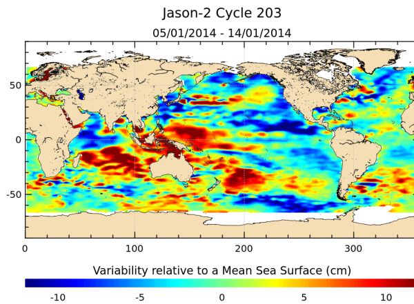
FIGURE 17 – Sea level anomaly relative to MSS for cycle 203.
