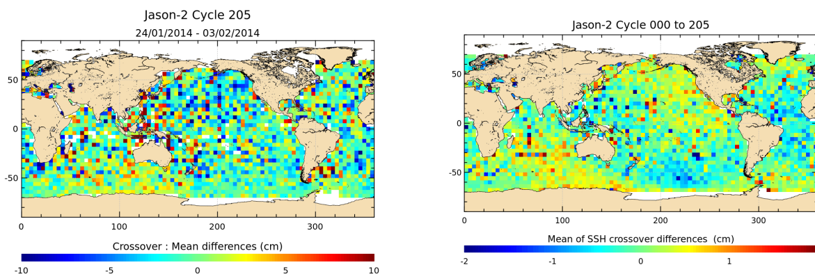
FIGURE 12 – Mean SSH at crossovers for cycle 205 (left) and over the whole Jason-2 period (right).
