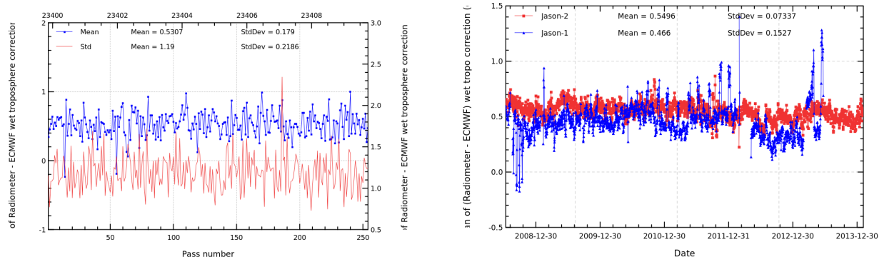
FIGURE 11 – Pass monitoring of wet troposphere differences between radiometer and ECMWF model for Jason-2 cycle 205 (left) and daily monitoring of wet troposphere differences between radiometer and ECMWF model (right).
