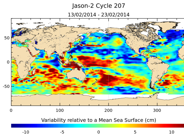
FIGURE 17 – Sea level anomaly relative to MSS for cycle 207.
