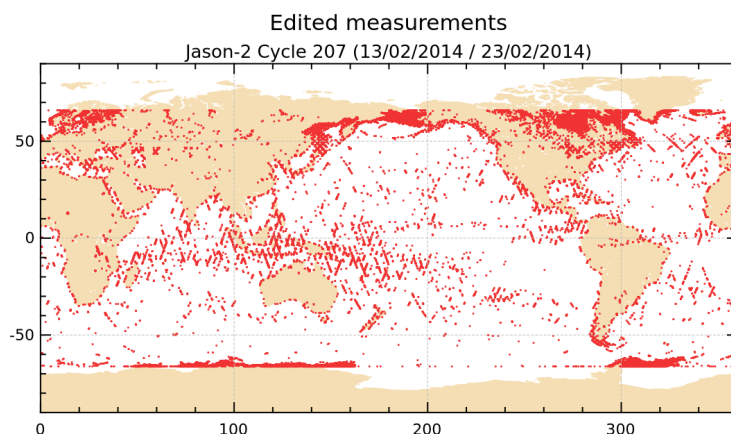
FIGURE 2 – Edited measurements for cycle 207.
