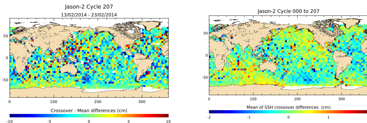
FIGURE 12 – Mean SSH at crossovers for cycle 207 (left) and over the whole Jason-2 period (right).
