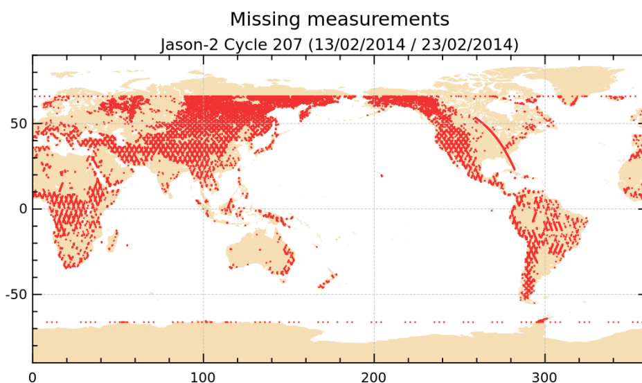
FIGURE 1 – Missing measurements for cycle 207.
