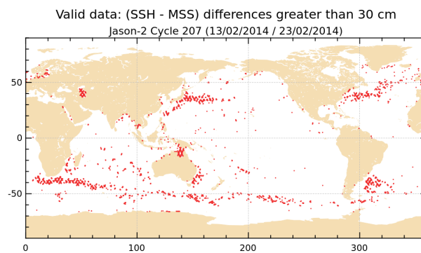
FIGURE 18 – Differences higher than a 30 cm threshold for cycle 207.
