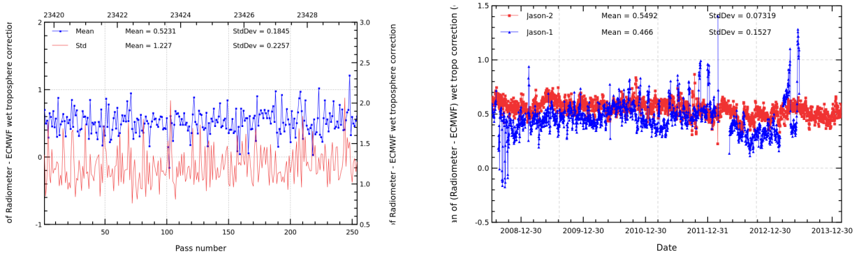
FIGURE 11 – Pass monitoring of wet troposphere differences between radiometer and ECMWF model for Jason-2 cycle 207 (left) and daily monitoring of wet troposphere differences between radiometer and ECMWF model (right).
