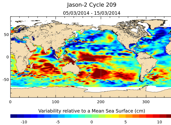
FIGURE 17 – Sea level anomaly relative to MSS for cycle 209.
