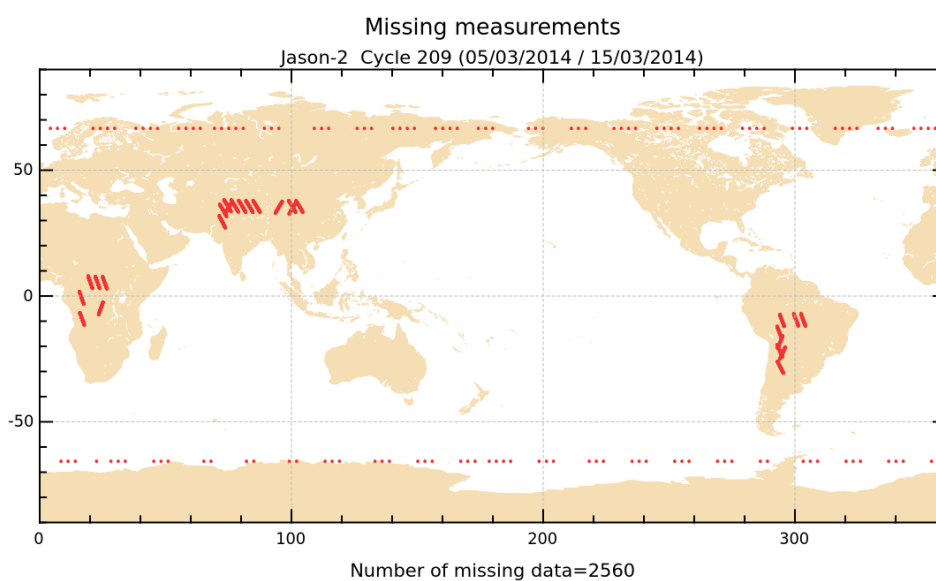
FIGURE 1 – Missing measurements for cycle 209.
