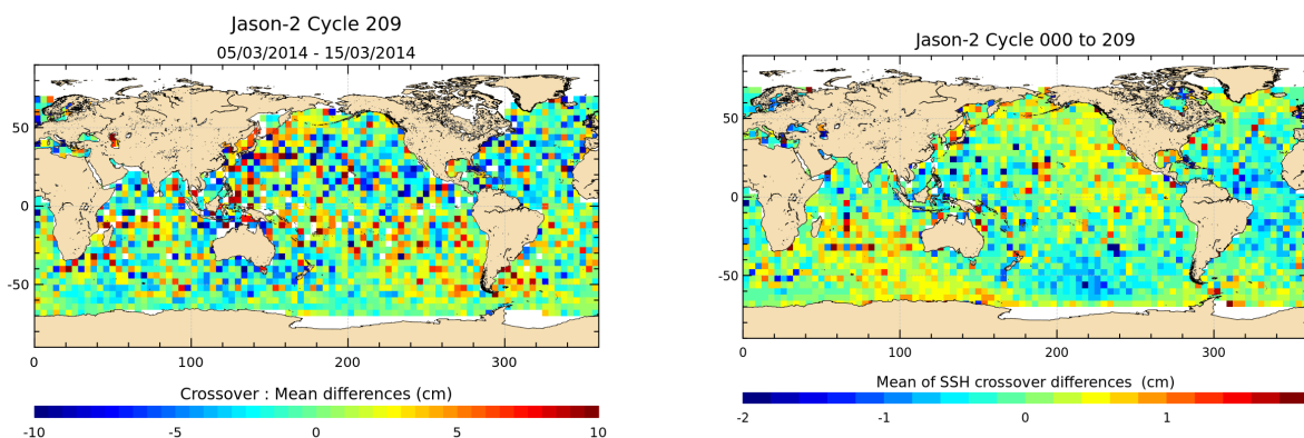
FIGURE 12 – Mean SSH at crossovers for cycle 209 (left) and over the whole Jason-2 period (right).
