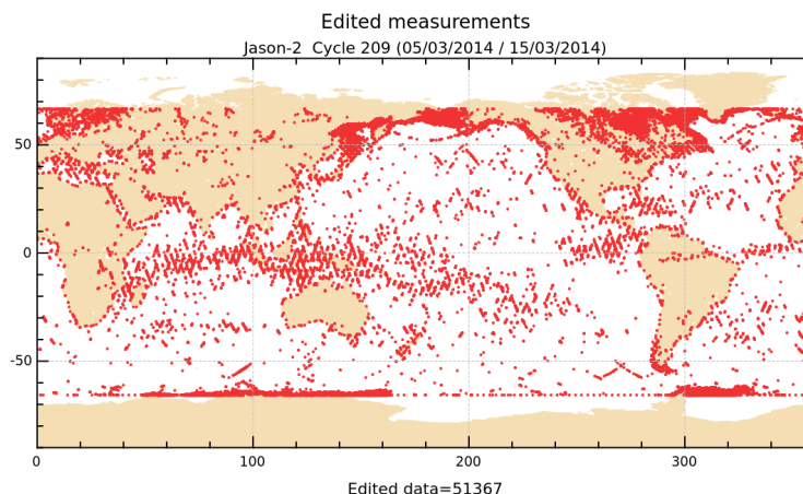
FIGURE 2 – Edited measurements for cycle 209.
