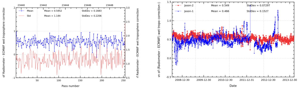
FIGURE 11 – Pass monitoring of wet troposphere differences between radiometer and ECMWF model for Jason-2 cycle 209 (left) and daily monitoring of wet troposphere differences between radiometer and ECMWF model (right).
