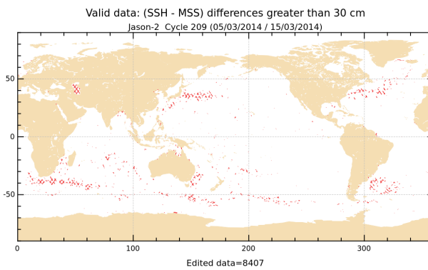
FIGURE 18 – Differences higher than a 30 cm threshold for cycle 209.
