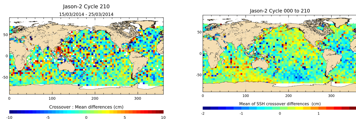
FIGURE 12 – Mean SSH at crossovers for cycle 210 (left) and over the whole Jason-2 period (right).
