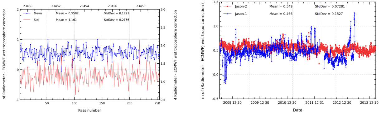
FIGURE 11 – Pass monitoring of wet troposphere differences between radiometer and ECMWF model for Jason-2 cycle 210 (left) and daily monitoring of wet troposphere differences between radiometer and ECMWF model (right).
