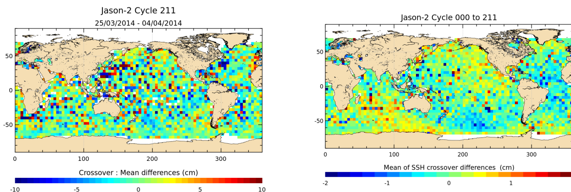
FIGURE 12 – Mean SSH at crossovers for cycle 211 (left) and over the whole Jason-2 period (right).
