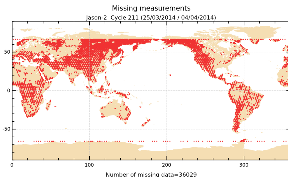
FIGURE 1 – Missing measurements for cycle 211.
