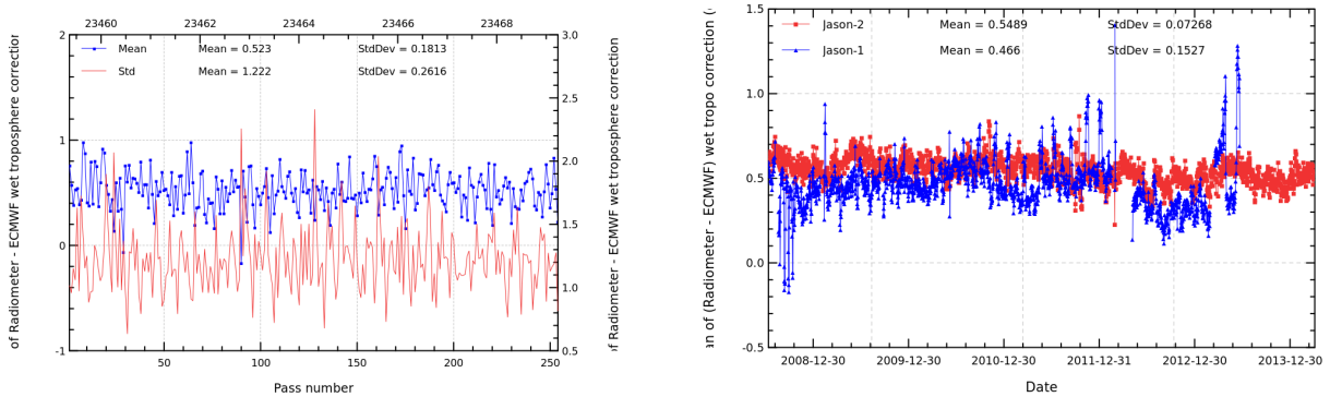
FIGURE 11 – Pass monitoring of wet troposphere differences between radiometer and ECMWF model for Jason-2 cycle 211 (left) and daily monitoring of wet troposphere differences between radiometer and ECMWF model (right).
