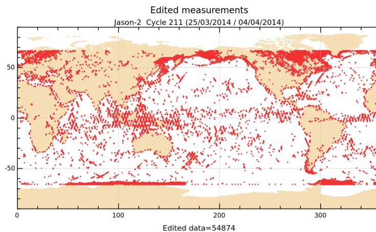
FIGURE 2 – Edited measurements for cycle 211.
