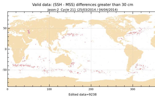
FIGURE 18 – Differences higher than a 30 cm threshold for cycle 211.
