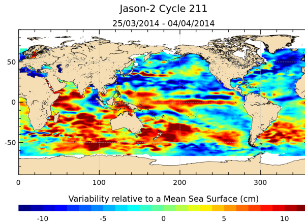
FIGURE 17 – Sea level anomaly relative to MSS for cycle 211.
