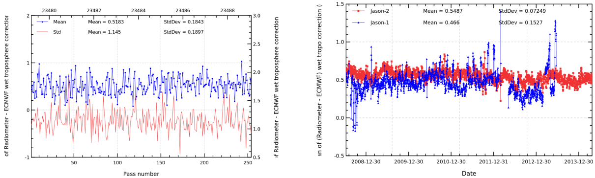
FIGURE 11 – Pass monitoring of wet troposphere differences between radiometer and ECMWF model for Jason-2 cycle 213 (left) and daily monitoring of wet troposphere differences between radiometer and ECMWF model (right).
