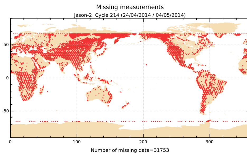
FIGURE 1 – Missing measurements for cycle 214.
