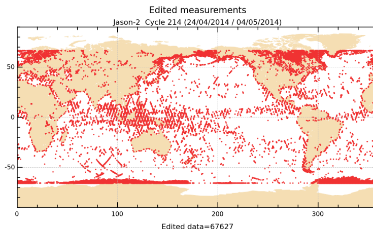
FIGURE 2 – Edited measurements for cycle 214.
