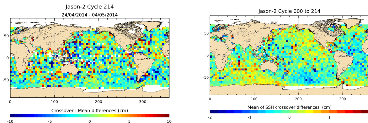
FIGURE 12 – Mean SSH at crossovers for cycle 214 (left) and over the whole Jason-2 period (right).
