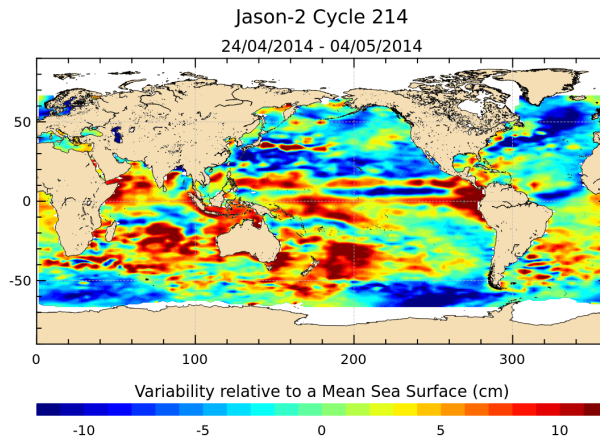
FIGURE 17 – Sea level anomaly relative to MSS for cycle 214.
