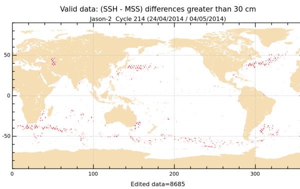
FIGURE 18 – Differences higher than a 30 cm threshold for cycle 214.
