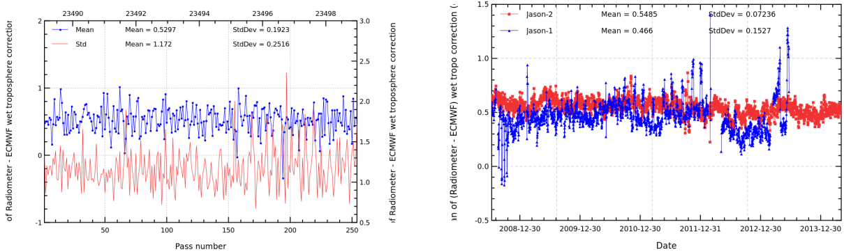
FIGURE 11 – Pass monitoring of wet troposphere differences between radiometer and ECMWF model for Jason-2 cycle 214 (left) and daily monitoring of wet troposphere differences between radiometer and ECMWF model (right).
