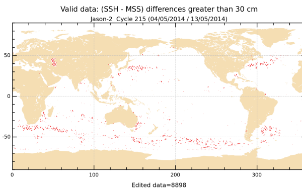
FIGURE 18 – Differences higher than a 30 cm threshold for cycle 215.
