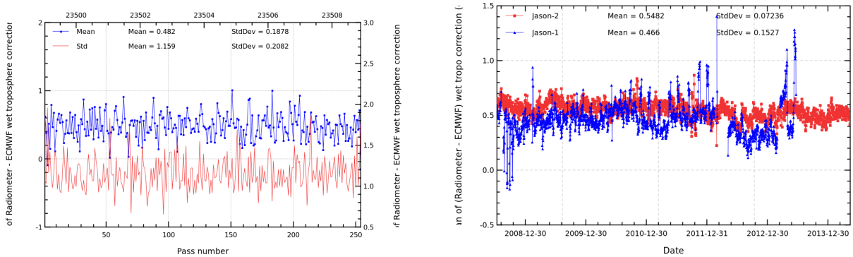
FIGURE 11 – Pass monitoring of wet troposphere differences between radiometer and ECMWF model for Jason-2 cycle 215 (left) and daily monitoring of wet troposphere differences between radiometer and ECMWF model (right).
