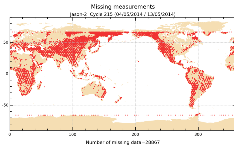
FIGURE 1 – Missing measurements for cycle 215.
