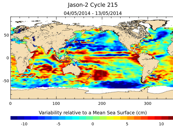
FIGURE 17 – Sea level anomaly relative to MSS for cycle 215.
