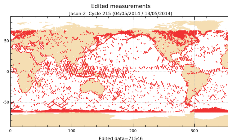
FIGURE 2 – Edited measurements for cycle 215.
