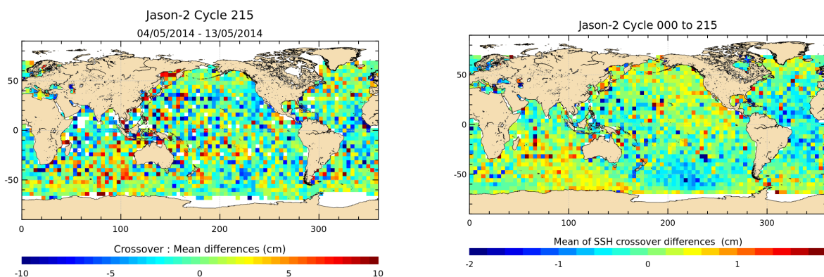
FIGURE 12 – Mean SSH at crossovers for cycle 215 (left) and over the whole Jason-2 period (right).
