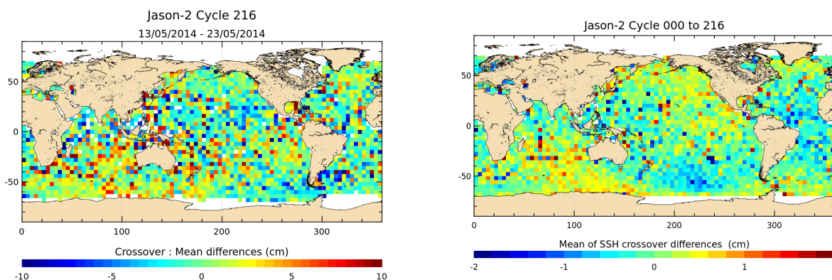
FIGURE 12 – Mean SSH at crossovers for cycle 216 (left) and over the whole Jason-2 period (right).
