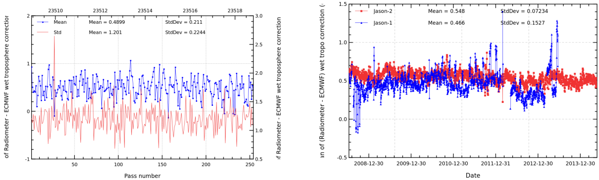
FIGURE 11 – Pass monitoring of wet troposphere differences between radiometer and ECMWF model for Jason-2 cycle 216 (left) and daily monitoring of wet troposphere differences between radiometer and ECMWF model (right).
