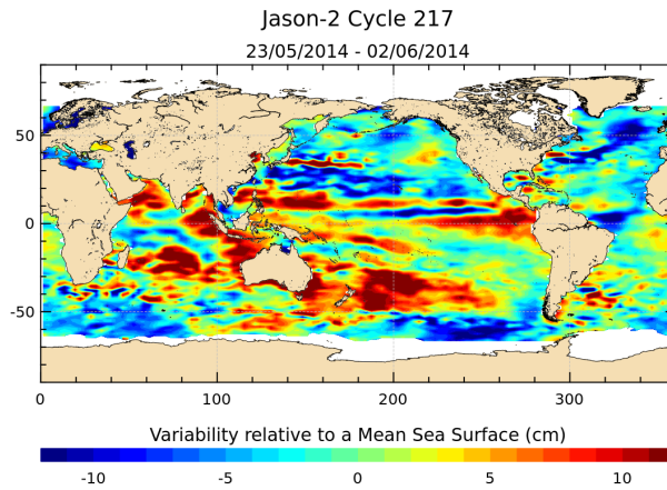
FIGURE 17 – Sea level anomaly relative to MSS for cycle 217.
