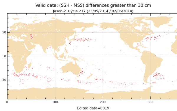
FIGURE 18 – Differences higher than a 30 cm threshold for cycle 217.
