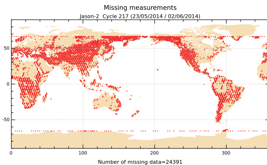
FIGURE 1 – Missing measurements for cycle 217.
