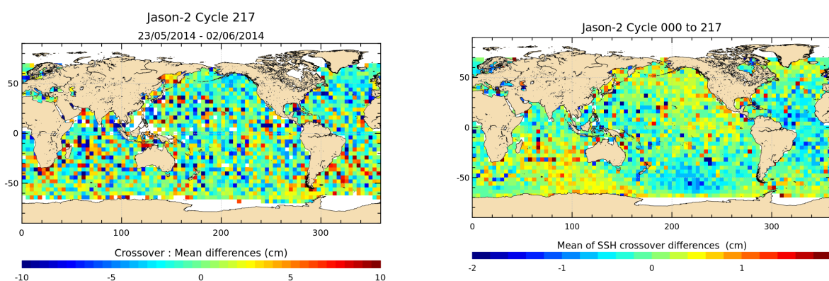
FIGURE 12 – Mean SSH at crossovers for cycle 217 (left) and over the whole Jason-2 period (right).
