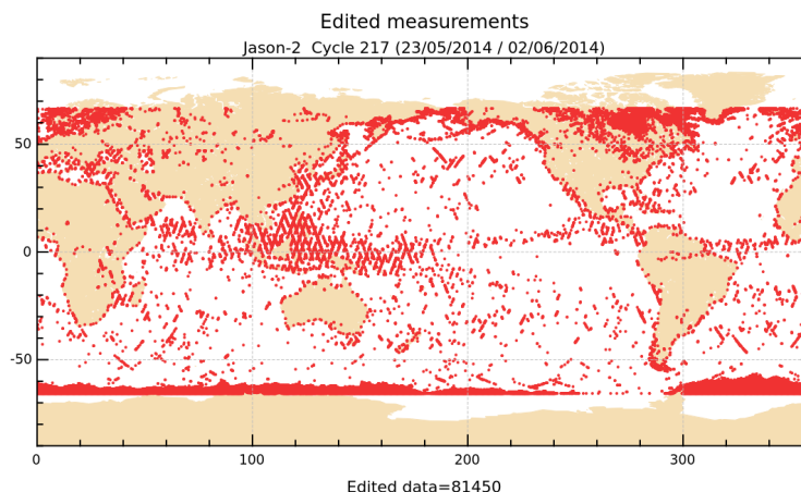
FIGURE 2 – Edited measurements for cycle 217.
