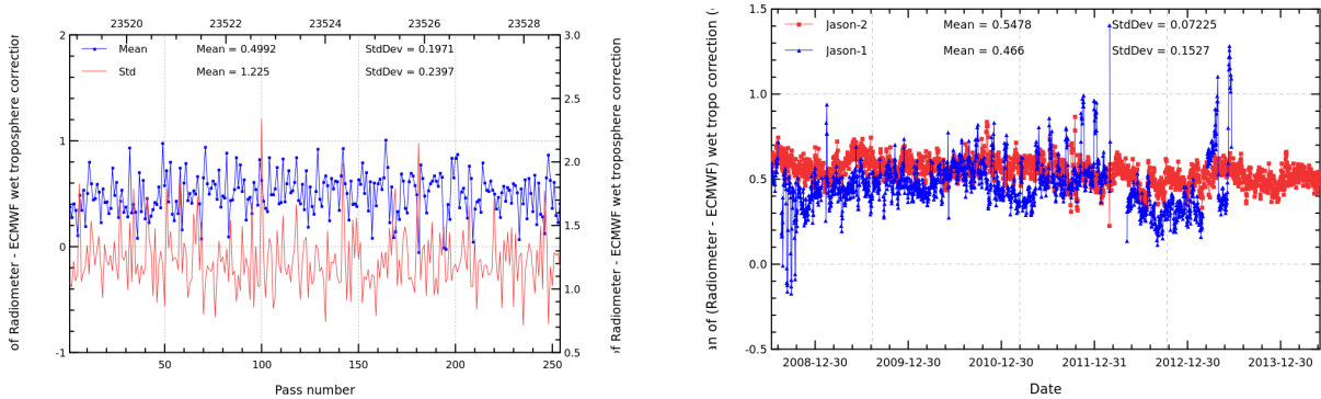
FIGURE 11 – Pass monitoring of wet troposphere differences between radiometer and ECMWF model for Jason-2 cycle 217 (left) and daily monitoring of wet troposphere differences between radiometer and ECMWF model (right).
