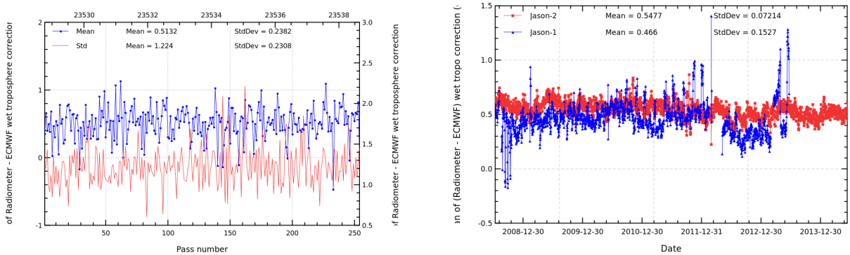
FIGURE 11 – Pass monitoring of wet troposphere differences between radiometer and ECMWF model for Jason-2 cycle 218 (left) and daily monitoring of wet troposphere differences between radiometer and ECMWF model (right).
