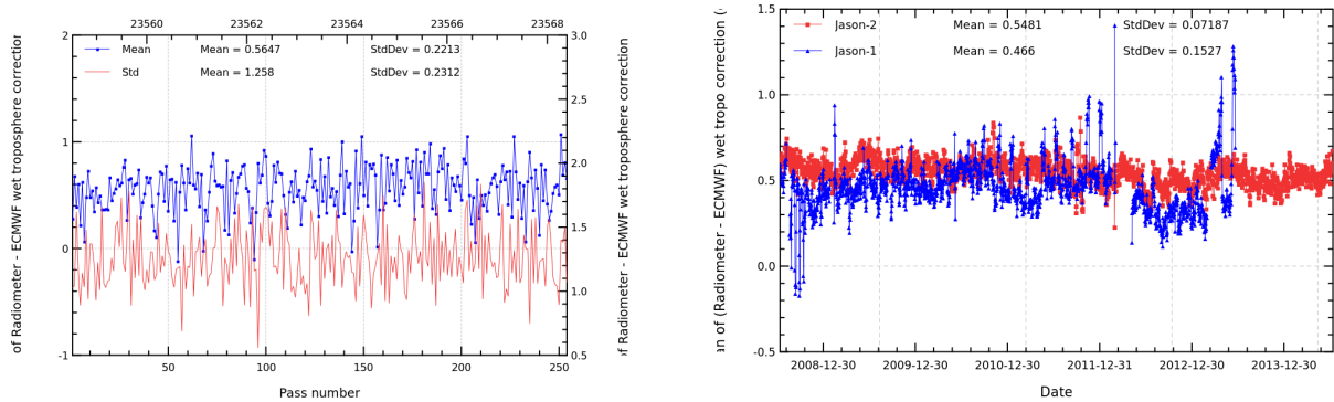
FIGURE 11 – Pass monitoring of wet troposphere differences between radiometer and ECMWF model for Jason-2 cycle 221 (left) and daily monitoring of wet troposphere differences between radiometer and ECMWF model (right).
