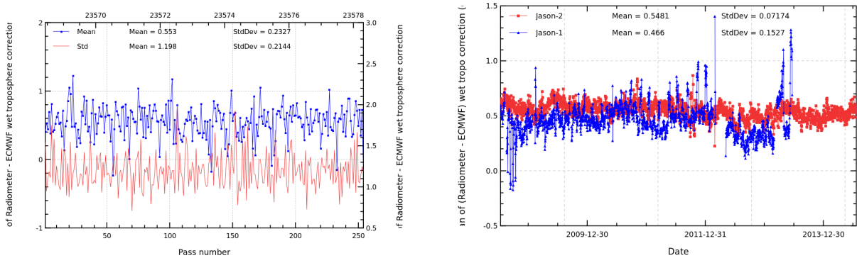
FIGURE 11 – Pass monitoring of wet troposphere differences between radiometer and ECMWF model for Jason-2 cycle 222 (left) and daily monitoring of wet troposphere differences between radiometer and ECMWF model (right).
