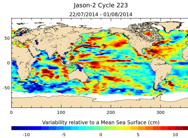
FIGURE 17 – Sea level anomaly relative to MSS for cycle 223.
