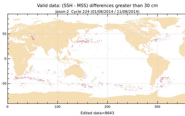
FIGURE 18 – Differences higher than a 30 cm threshold for cycle 224.
