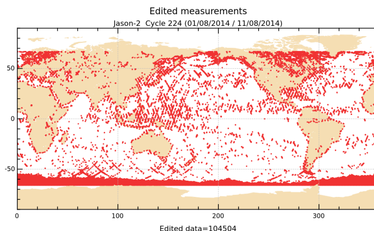
FIGURE 2 – Edited measurements for cycle 224.
