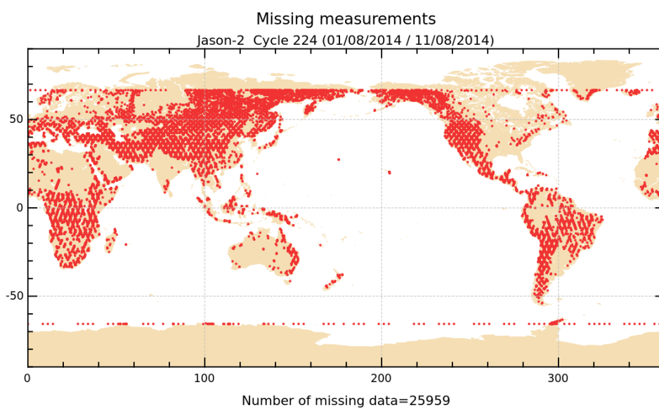
FIGURE 1 – Missing measurements for cycle 224.
