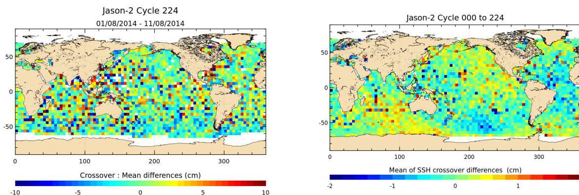
FIGURE 12 – Mean SSH at crossovers for cycle 224 (left) and over the whole Jason-2 period (right).
