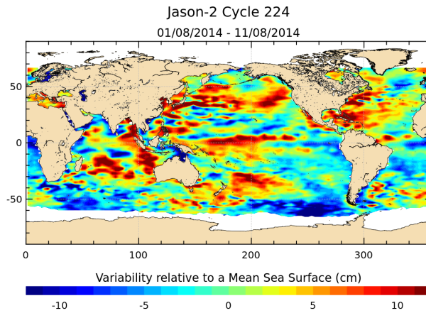
FIGURE 17 – Sea level anomaly relative to MSS for cycle 224.
