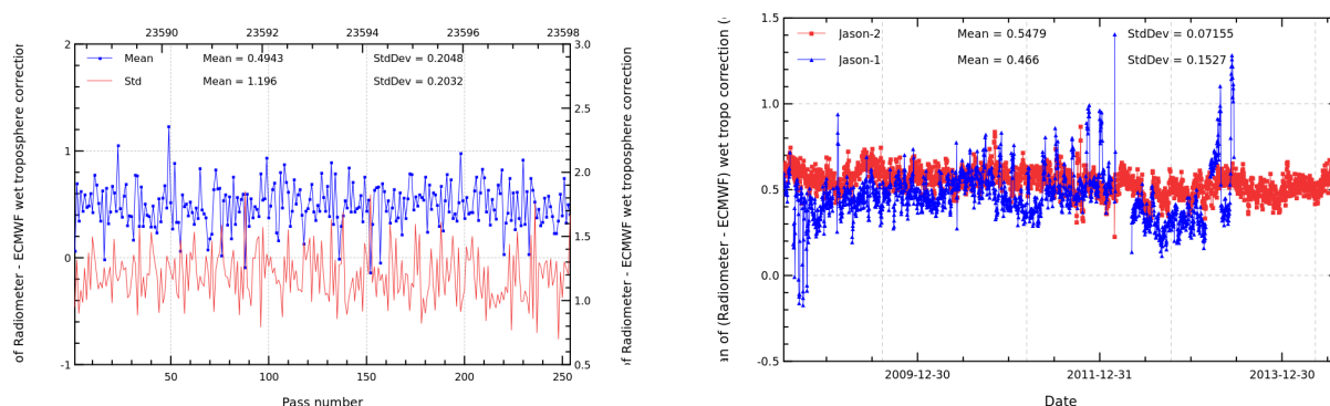
FIGURE 11 – Pass monitoring of wet troposphere differences between radiometer and ECMWF model for Jason-2 cycle 224 (left) and daily monitoring of wet troposphere differences between radiometer and ECMWF model (right).
