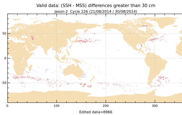
FIGURE 18 – Differences higher than a 30 cm threshold for cycle 226.
