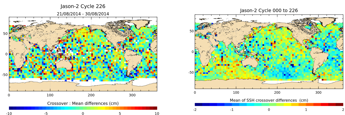
FIGURE 12 – Mean SSH at crossovers for cycle 226 (left) and over the whole Jason-2 period (right).
