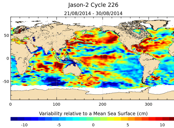
FIGURE 17 – Sea level anomaly relative to MSS for cycle 226.
