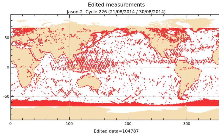
FIGURE 2 – Edited measurements for cycle 226.
