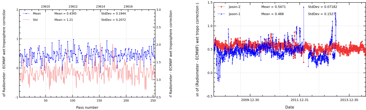
FIGURE 11 – Pass monitoring of wet troposphere differences between radiometer and ECMWF model for Jason-2 cycle 226 (left) and daily monitoring of wet troposphere differences between radiometer and ECMWF model (right).
