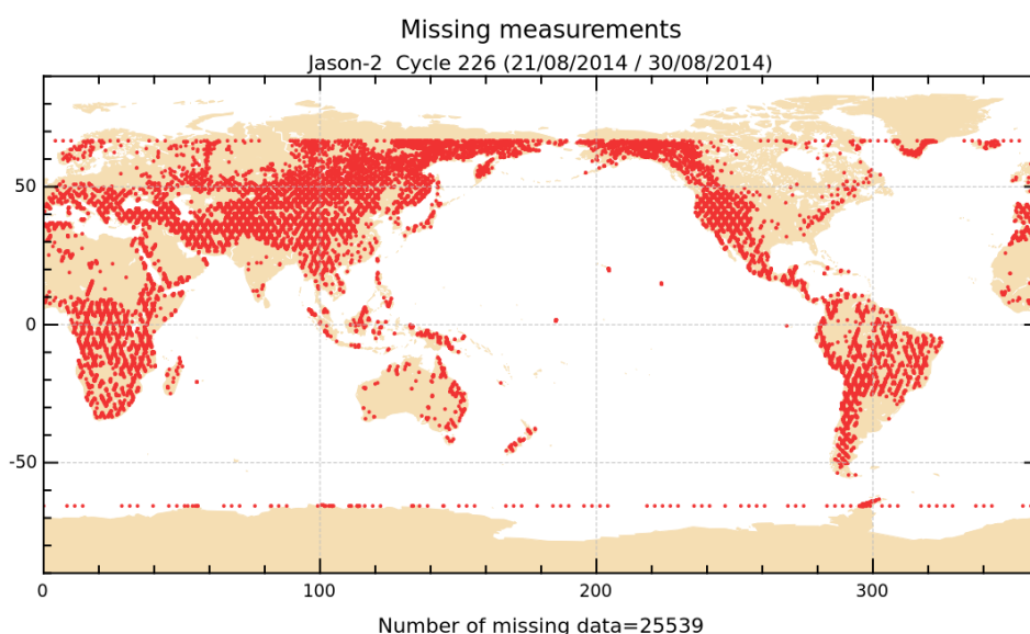
FIGURE 1 – Missing measurements for cycle 226.
